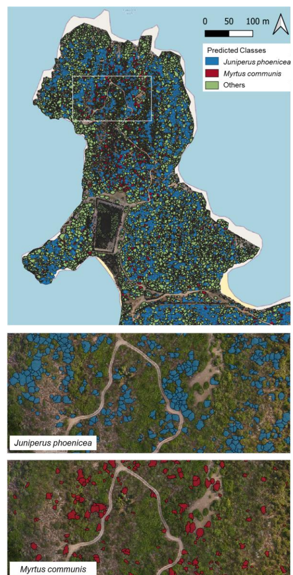
Figure 8. Spatial classification map of vegetation species across Culuccia Island, illustrating the predicted distribution of Juniperus phoenicea , Myrtus communis , and other vegetation classes, with zoomed-in examples of classified Juniper and Myrtle species in the northern part of the island.
