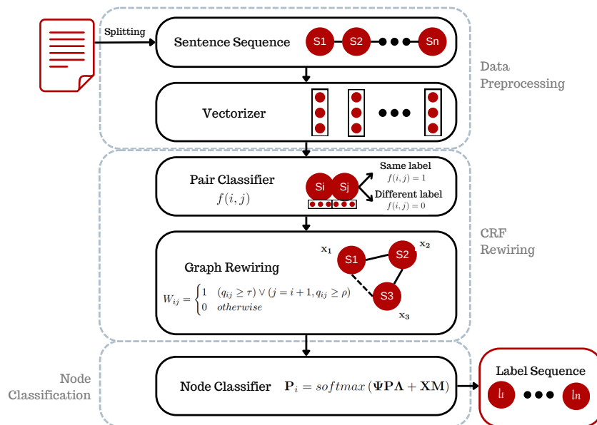
Figure 2: Few-shot functional Text Segmentation model.
