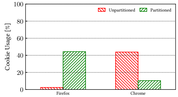
(b) After-Deny
