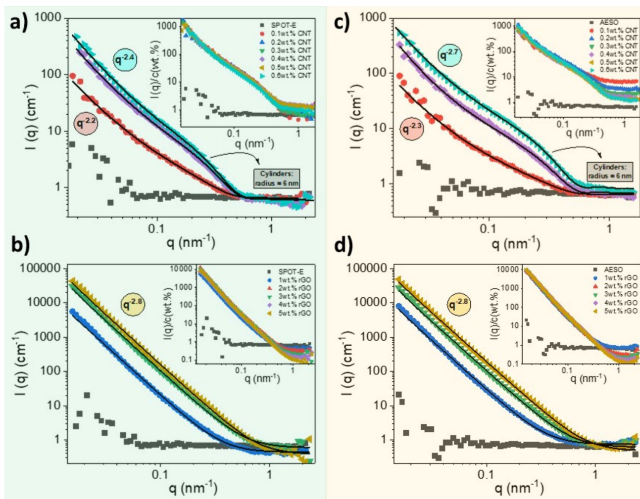
Fig. 4 Experimental SANS plots for pristine and SPOT-E and AESO composites containing CNT (a and c, respectively) and rGO (b and d, respectively). Inset figures of (a–d) plot the SANS curves normalized
