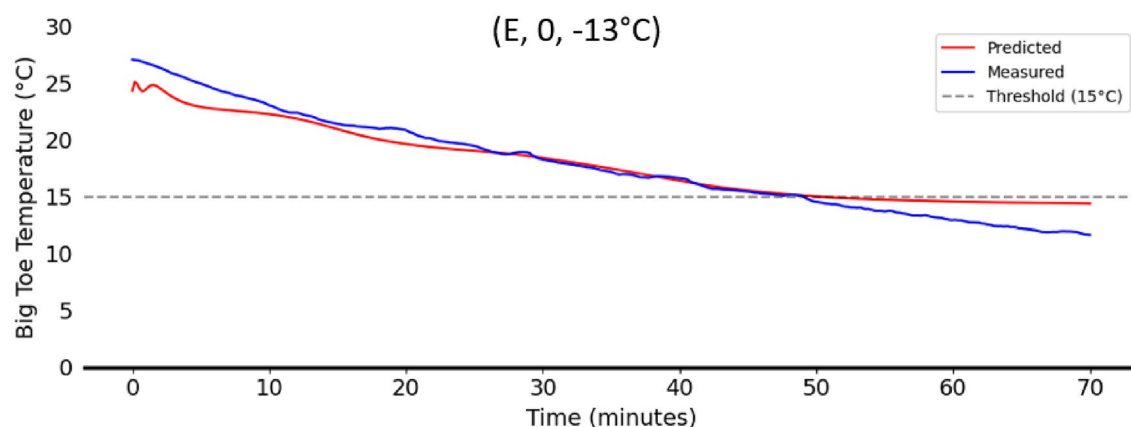
Fig. 5. Representative example of accurate LSTM predictions. The network successfully captures both the shape of the temperature curve and the timing of the threshold-crossing event.
