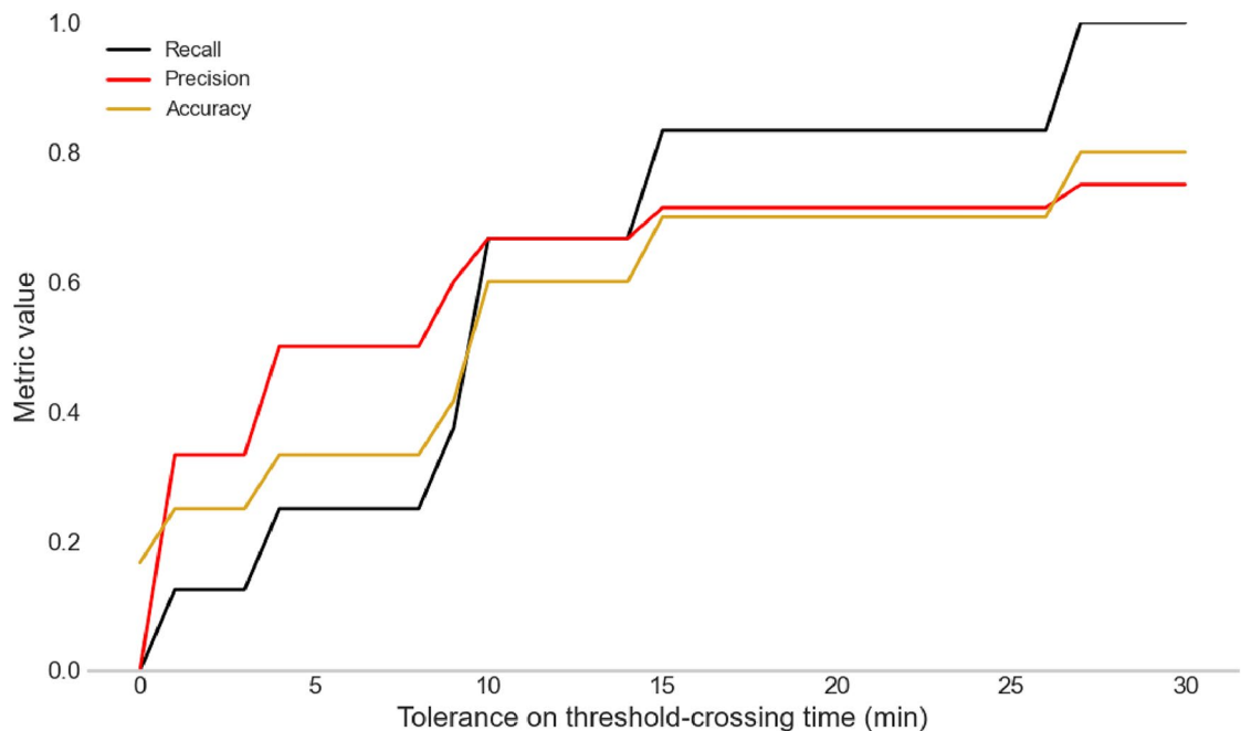
Fig. 3. Time-to-event tolerance curve for the threshold-crossing prediction. Accuracy, precision, and recall are shown as a function of the temporal tolerance \tau applied to the predicted crossing time.
