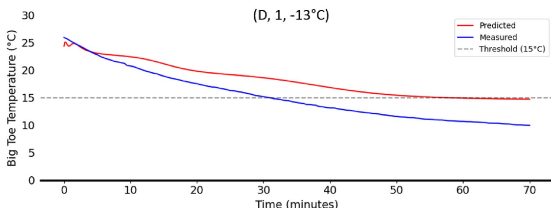
Fig. 6. Example of inaccurate prediction performance. The threshold crossing was not identified, although the overall temperature trajectory was correctly reproduced.
