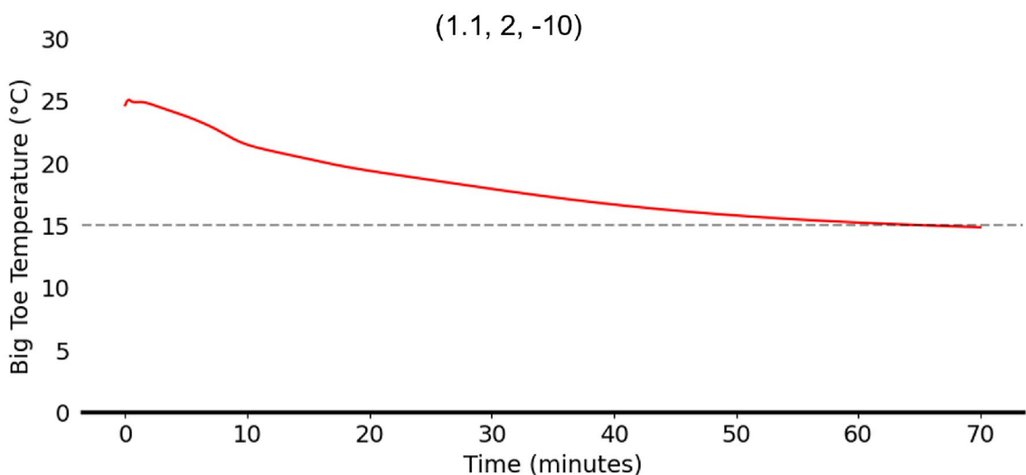
Fig. 10. LSTM prediction under high physical activity with reduced boot insulation ( R_{cT} = 1.1 ) at -10^{\circ}\text{C} . The predicted time to threshold is 64 minutes.
