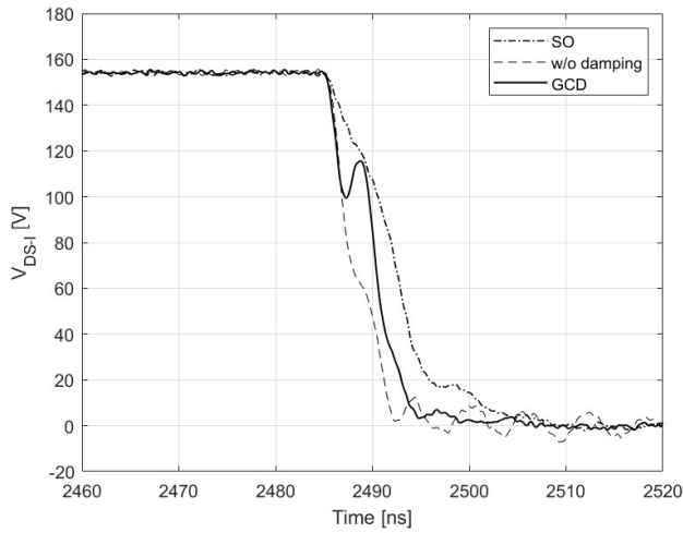
Fig. 7. V_{DS-l} with dpt: maximum speed, SO control, GCD technique.
