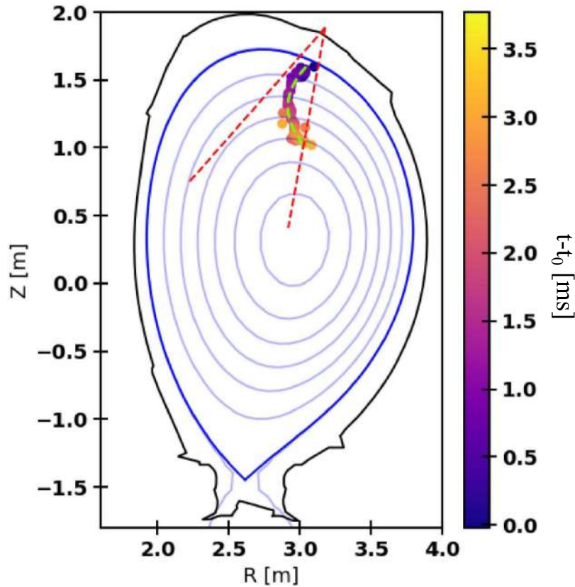
Figure 15. Tracked inboard edge of the SPI plume based on the maximum gradient of the D_{\alpha} emission intensity detected by the KL8 fast camera in JET # 96874. Time in milliseconds shown in the colorbar is shifted by t_0 = 9.039 s, i.e. the time when the first group of fragments arrive at the plasma. Outlines of the expected SPI plume from the injection geometry are shown by the red dashed lines. Reproduced from [102]. The Author(s). CC BY 4.0.
