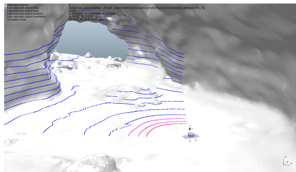
Figure 3. CoppeliaSim setup.
