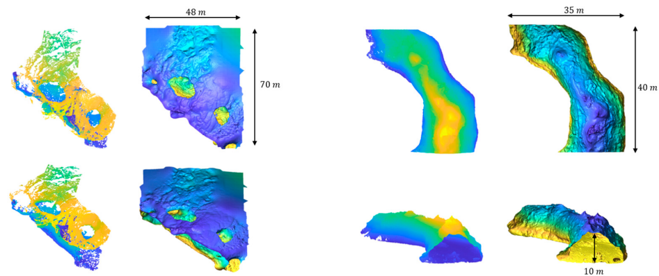
Figure 2. Point clouds of craters and tunnels—source NASA.
