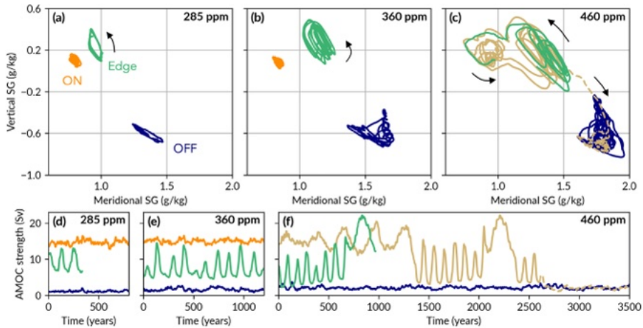
Figure 11. AMOC stability landscape as function of CO 2 concentration for 285 ppm (a,d), 360 ppm (b,e) and 460 ppm (c,f). Reduced state space projections (a–c) onto the meridional and vertical SG show the ON (orange), OFF (blue) and edge trajectory (green). For 460 ppm, the transient trajectory initialized from the former ON state (beige) and the edge trajectory (green) trace the ghost state. Arrows indicate the time direction. (d–f) AMOC timeseries at 46–66°N corresponding to (a–c), respectively.
