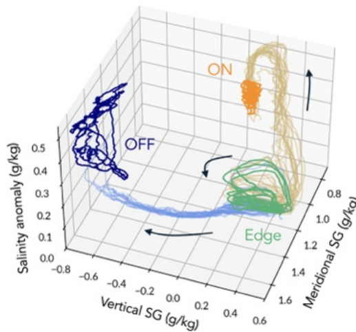
Figure 6. State space projection onto the meridional SG, vertical SG, and deep North Atlantic salinity anomaly (below 1000 m, north of 50^{\circ}\text{S} ). Faint orange (blue) lines show trajectories relaxing from near the edge state to the ON (OFF) state. Arrows indicate the time direction.
