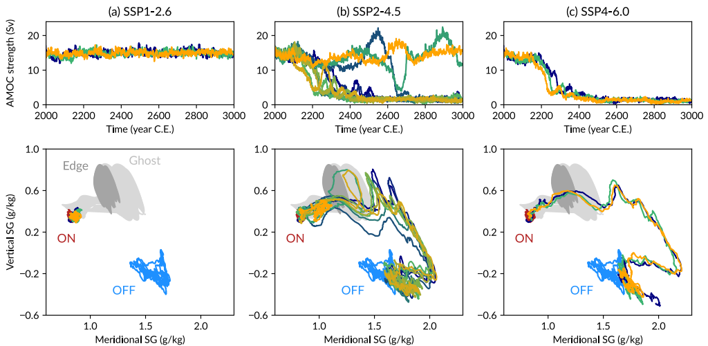
Figure 13. Trajectories of PlaSim-LSG under future CO 2 emission scenarios for ensemble members run under the (a) SSP1–2.6, (b) SSP2–4.5 and (c) SSP4–6.0 scenario. Top panels show the AMOC timeseries, bottom panels show their projection onto the reduced state space spanned by the meridional and vertical SG. Dark and light grey shaded areas indicate the region of the edge state at 360 ppm and ghost state at 460 ppm, respectively. The ON (red) and OFF (blue) states at 360 ppm are shown for reference.
