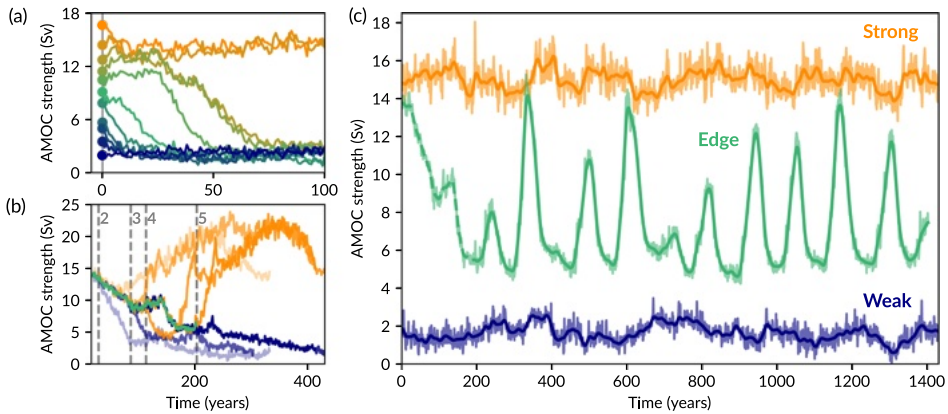
Figure 5. Edge tracking and AMOC states at 360ppm CO 2 . (a) Interpolating initial conditions between the ON (orange) and OFF (blue) AMOC state allows locating the basin boundary. (b) Iterations 2–5 of the edge tracking algorithm, showing the trajectories that converge to ON (orange) and OFF (blue), respectively. The edge pseudotrajectory (green) is constructed from segments of these trajectories. (c) Edge trajectory (green) and trajectories on the ON (orange) and OFF (blue) attractors. The AMOC strength is measured between 46°N and 66°N.
