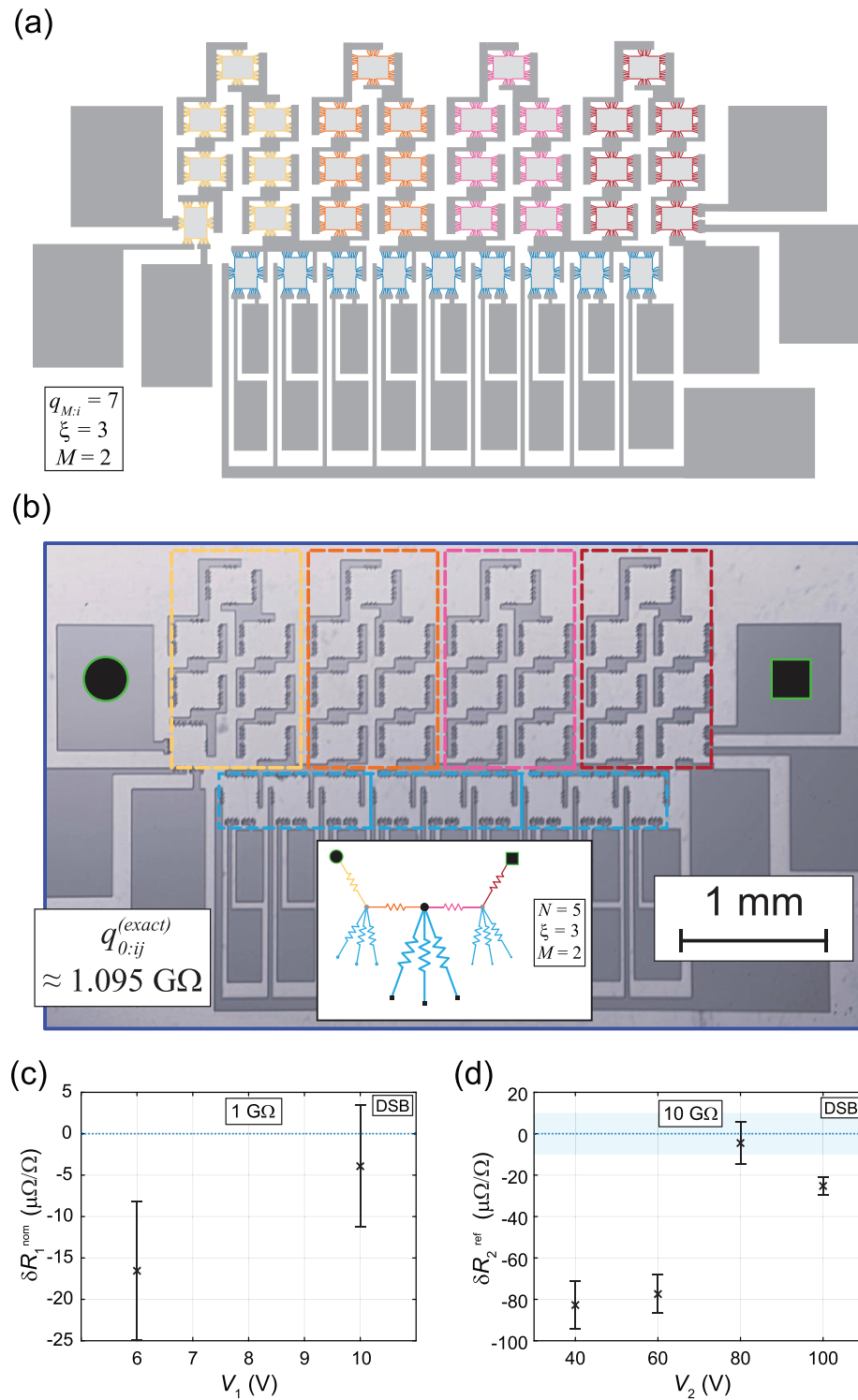
Figure 2. (a) QHARS device design layout with corresponding parameters M=2 , \xi=3 , and q_{M;i}=7 . (b) Device post-fabrication optical image, overlaid by color-coded markers that match with those in the central inset showing a simplified network drawing presented in the style of [8]. (c) DSB data are shown to verify that the QHARS device is quantized (that is, each of its elements are successfully exhibiting the quantum Hall effect with high precision), with a standard resistor serving as the known quantity. The deviation from nominal \delta R_1 is centered around q_{0:ij}^{(exact)} = 1.095069 \dots \text{ G}\Omega . Error bars represent a 1\sigma uncertainty. (d) More DSB data denote the utility in using QHARS devices for calibrations at 10 \text{ G}\Omega . The highlighted blue is the 1\sigma uncertainty on the value of the standard resistor and the data points are the determined value of the same resistor using the QHARS device, with error bars representing 1\sigma uncertainty.
