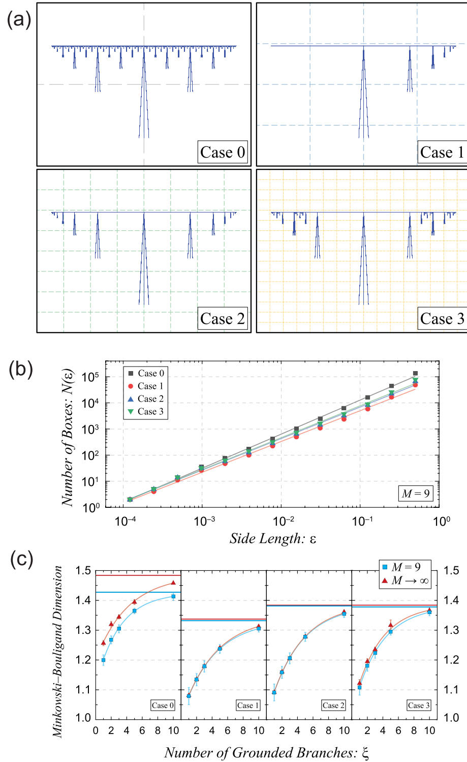
Figure 3. (a) This illustration depicts the four distinct pseudofractals used for the cases in the relevant calculations. Each panel is accompanied by an example overlay of a single box-counting computation, where the boxes containing the pseudofractal are tracked as a function of box size. (b) The prior computations are tabulated and plotted on a log-log plot, whose resulting curves may be fit to a line whose slope reveals the Minkowski–Bouligand dimension of the relevant pseudofractal. Example pseudofractals from the M = 9 iterations of all four cases from (a) are plotted. (c) A summary of the MBDs for each pseudofractal are shown as a function of \xi , with two distinct curves for the same M = 9 iterations (in blue) and for the ideal case of the pseudofractal where the iterations approach infinity (in red).
