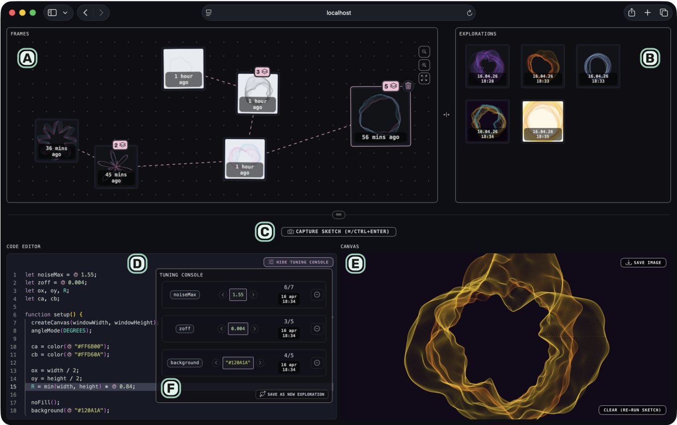
Figure 1: This article presents Reframe , a web-based Creative Coding environment for p5.js that rethinks versioning as a creative practice. The interface brings together non-linear navigation across frames and explorations, direct code editing, parameter-level exploration, and continuous visual feedback, supporting users in revisiting, comparing, and further developing evolving directions of a code-based artwork.
