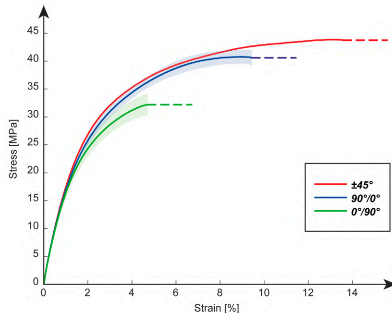
Figure 4. Average tensile test curves for the \pm 45^\circ , 0^\circ/90^\circ , and 90^\circ/0^\circ cases. The shaded area represents \pm 1 standard deviation calculated from the curves obtained from the five replicas. Average curves are reported up to the first-failure elongation for each batch.
