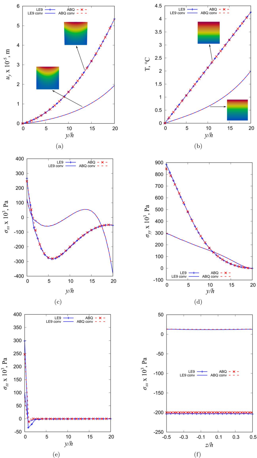
Figure 5. Comparison of present methodology with 3D abaqus solutions for the aluminum panel, considering scenarios with and without convection.
