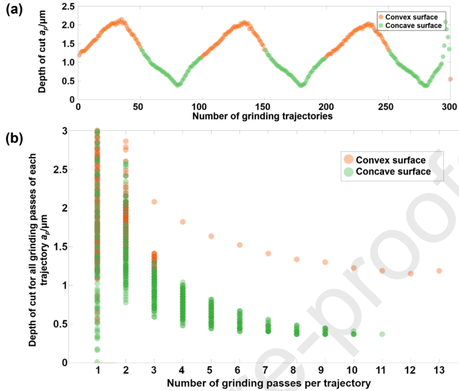
Figure 14 Grinding depth distribution ((a) the grinding depth of each grinding trajectory when closest to the surface (b) the full grinding depth of each grinding trajectory)
