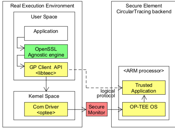
Fig. 1. Architectural overview of the proposed software stack, which redirects OpenSSL cryptographic operations to OP-TEE through the GP client Application Programming Interface (API).
