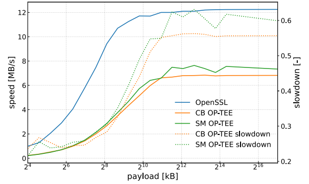
Fig. 3. Throughput of SHA-256 hashing for native OpenSSL, CB communication, and SM communication. Solid curves indicate throughput [MB/s]; dotted lines denote slowdown relative to native execution.
