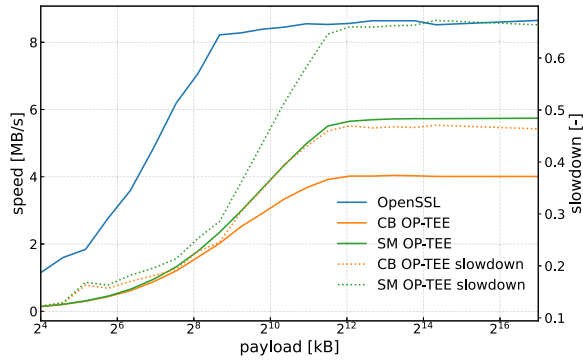
Fig. 4. Throughput of AES-256-CBC encryption for native OpenSSL, CB communication and SM communication. Solid curves indicate throughput [MB/s]; dotted lines denote slowdown relative to native execution.
