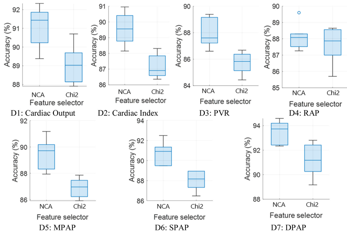
Figure 10. Classification accuracies by feature selector method for the seven datasets: D1. CO; D2. CI; D3. PVR; D4. RAP; D5. MPAP; D6. SPAP; D7: DPAP.
