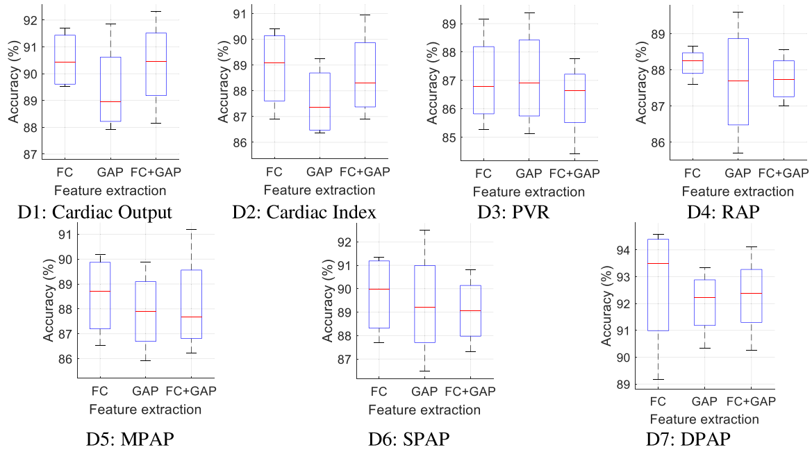
Figure 9. Classification accuracies by feature extraction method for the seven datasets: D1. CO; D2. CI; D3. PVR; D4. RAP; D5. MPAP; D6. SPAP; D7: DPAP.
