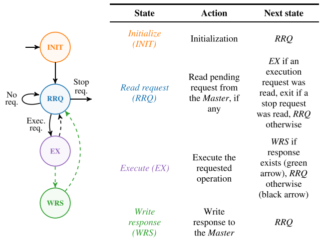
FIGURE 4. Finite-state machine summarizing the behavior of a Slave in our Cyclic dataflow protocol .
