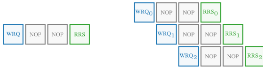
(a) Static schedule. (b) Runtime behavior.
