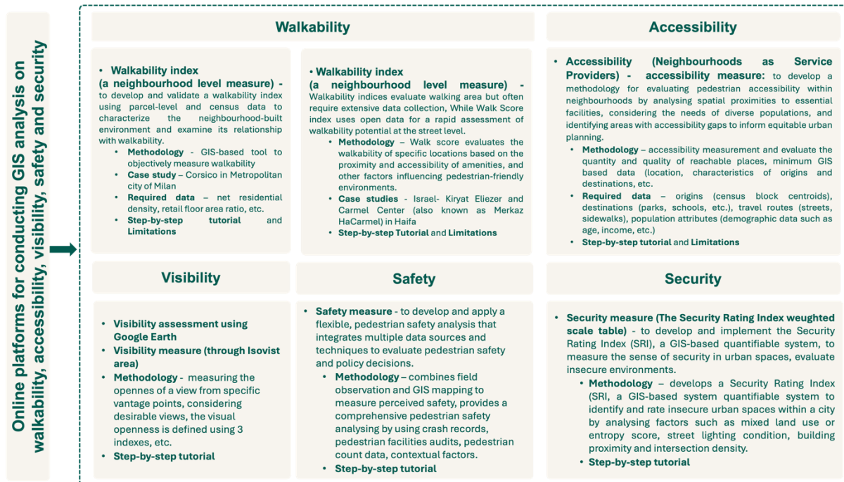
Figure 26. Workflow for online platforms for conducting GIS analysis.
