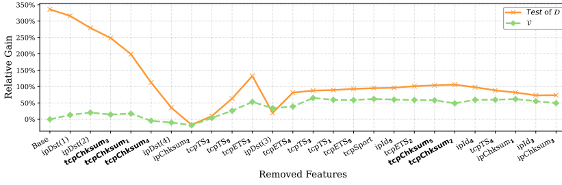
Fig. 4. SHORTCUTCATCHER applied to the RF classifier. Flow classification task on App-Time, scenario S_2 .
