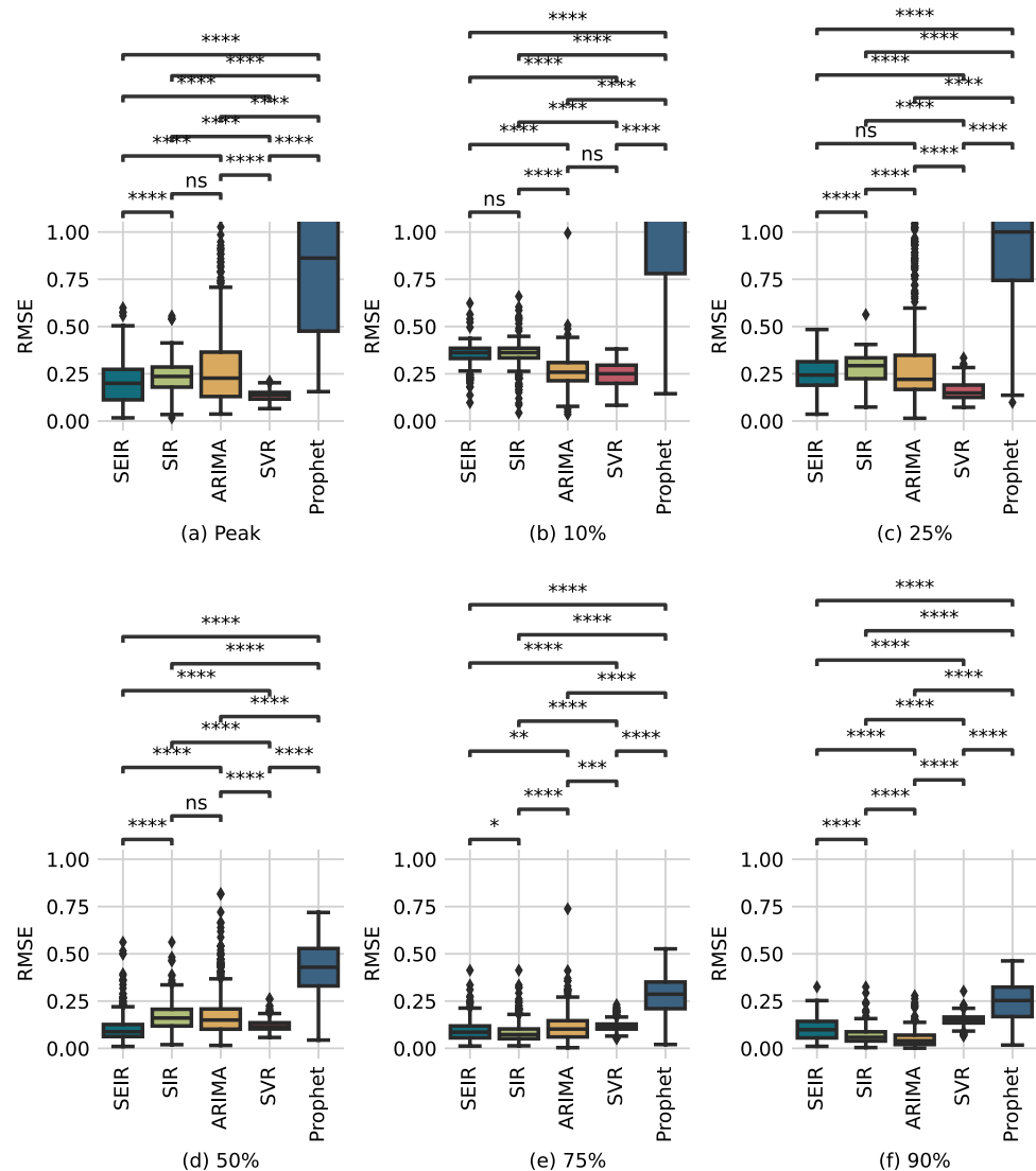
Fig. 8 Forecasting performance for our approach with base-lines. Significance is calculated using the Mann–Whitney U test: * for 0.01 < p \leq 0.05 ; ** for 0.001 < p \leq 0.01 ; *** for 0.0001 < p \leq 0.001 ; **** for p \leq 0.0001 and ‘ns’ for p > 0.05
