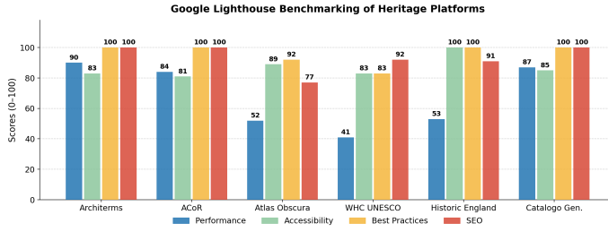
Fig. 2. Comparative analysis of the selected cultural heritage platforms based on Google Lighthouse performance indices. The benchmarking highlights the trade-offs between rich multimedia content and technical performance.
