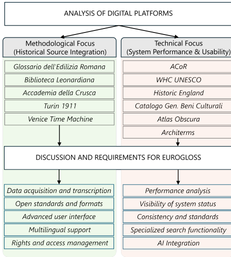
Fig. 1. Systematic analysis of digital platforms for the development of EUROGLOSS requirements.
