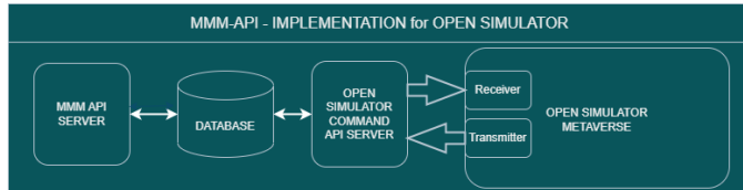
Fig. 3. Implementation of MMM-API for OPEN SIMULATOR.
