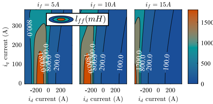
Fig. 22: Current-to-inductance l_{ff} map for the EESM under consideration.
