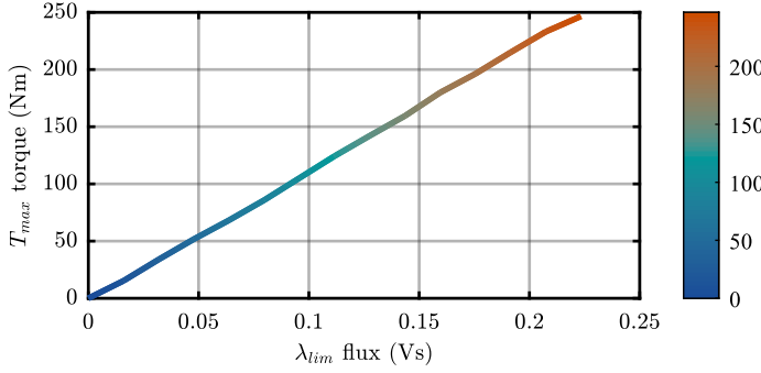
Fig. 9: Maximum torque ( T_{max} ) profile (LUT1) for the EESM under consideration.
