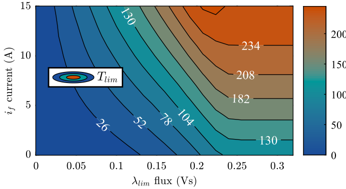
Fig. 10: Torque limit ( T_{lim} ) map (LUT2) for the EESM under consideration.
