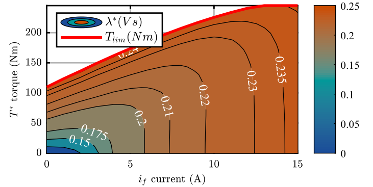
Fig. 12: Flux amplitude reference ( \lambda^* ) map (LUT3) for the EESM under consideration.
