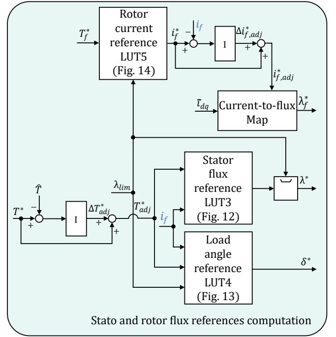
Fig. 11: Schematic view of the stator and rotor flux references computation.
