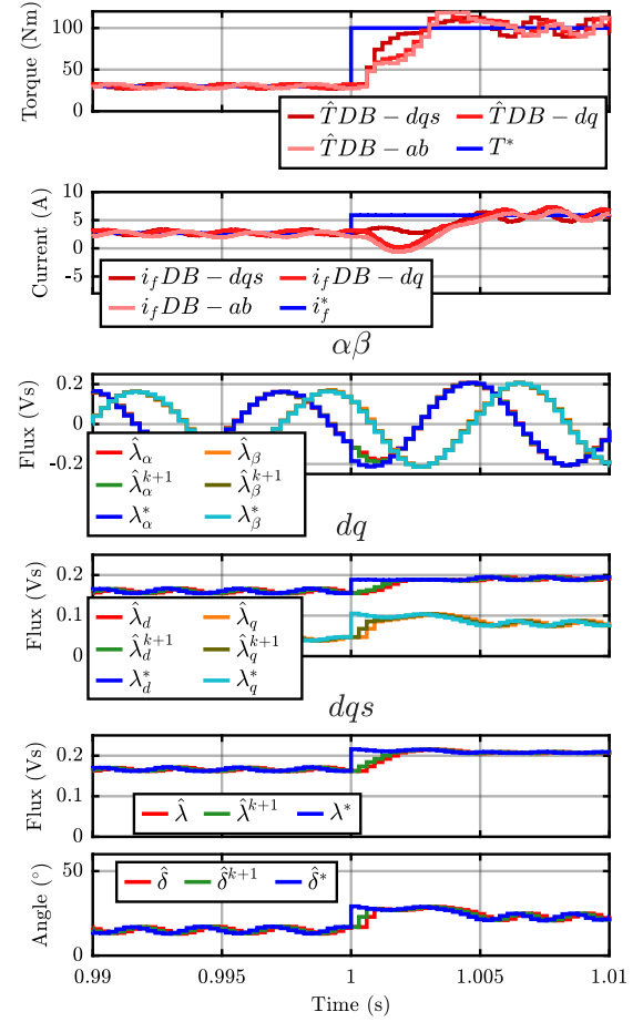
Fig. 25: Experimental results of torque step response from 30 to 100 Nm, 4000 r/min.
