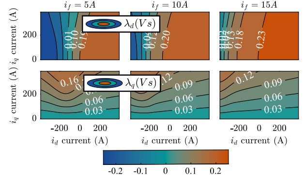
Fig. 5: Stator current-to-flux maps for the EESM under consideration.
