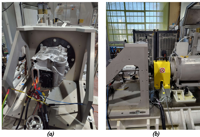
Fig. 19: View of the test rig: (a) EESM under test; (b) EESM coupled with the driving machine.
