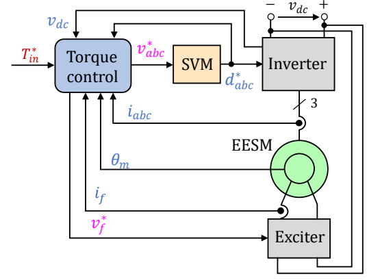
Fig. 1: Schematic view of the considered EESM drive topology.
