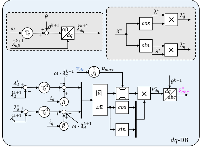
Fig. 16: Schematic view of the dq -frame based DB approach.
