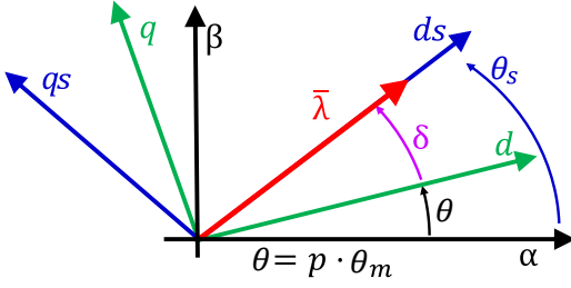
Fig. 2: Schematic view of the stationary- \alpha\beta , rotor- dq , and stator- dqs frames for a generic synchronous motor.
