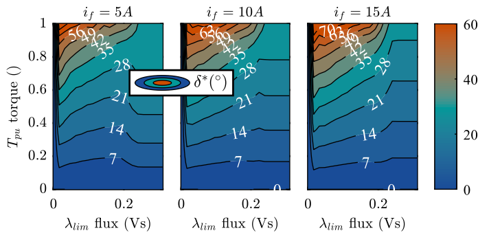
Fig. 32: Normalized load angle reference ( \delta^* ) map (LUT4) for the EESM under consideration.
