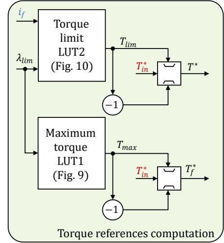
Fig. 8: Schematic view of the torque references computation.
