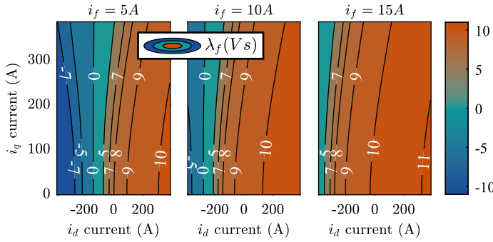
Fig. 7: Rotor current-to-flux maps for the EESM under consideration.
