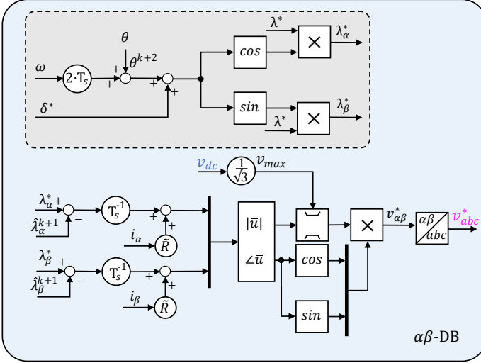
Fig. 15: Schematic view of the \alpha\beta -frame based DB approach.
