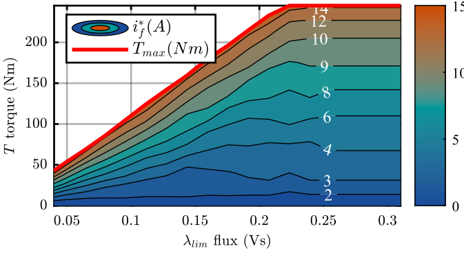
Fig. 14: Rotor current reference ( i_f^* ) map (LUT5) for the EESM under consideration.
