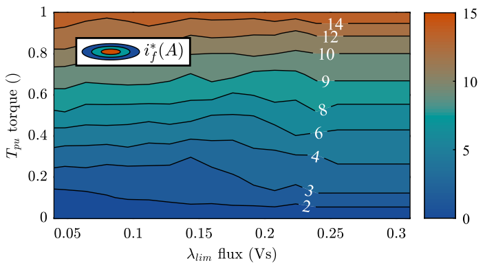
Fig. 33: Normalized rotor current reference ( i_f^* ) map (LUT5) for the EESM under consideration.
