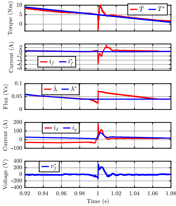
Fig. 26: Experimental results of torque transient from 50 to 0 Nm using DB-dqs, 50 Nm/s, 4000 r/min: magnification view of the stator dq currents and the reference rotor voltage v_f^* .
