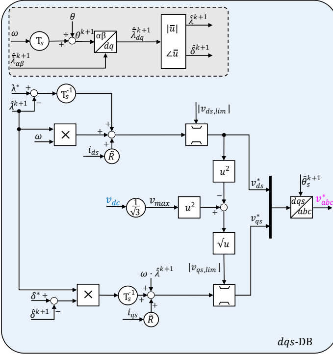
Fig. 17: Schematic view of the dqz -frame based DB approach.
