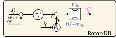
Fig. 18: Schematic view of the DB rotor flux regulator.
