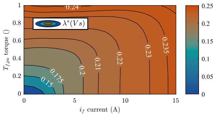
Fig. 31: Normalized flux amplitude reference ( \lambda^* ) map (LUT3) for the EESM under consideration.
