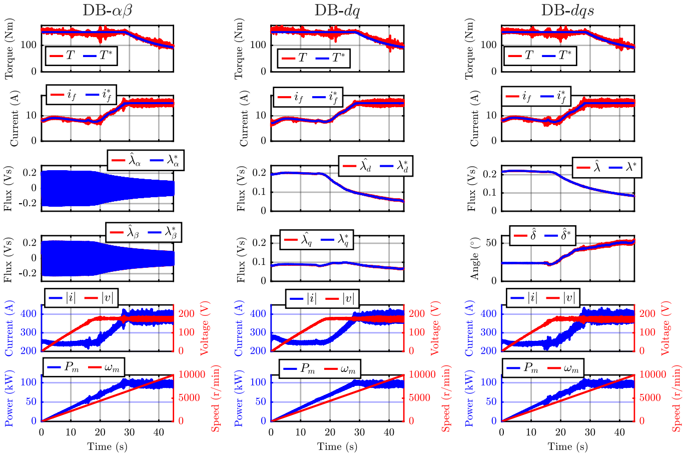
Fig. 20: MTPS profiles: experimental results.
