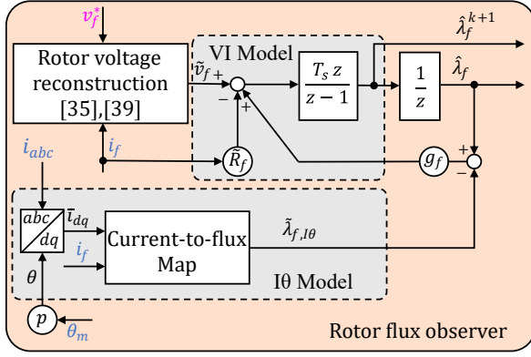
Fig. 6: Schematic view of the adopted rotor flux observer.
