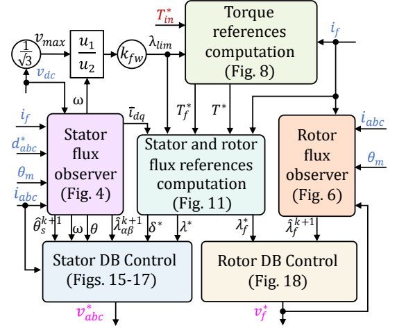
Fig. 3: Schematic view of the proposed torque controller.
