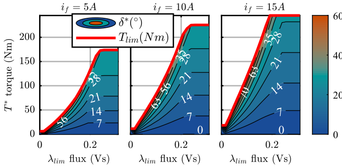
Fig. 13: Load angle reference ( \delta^* ) map (LUT4) for the EESM under consideration.
