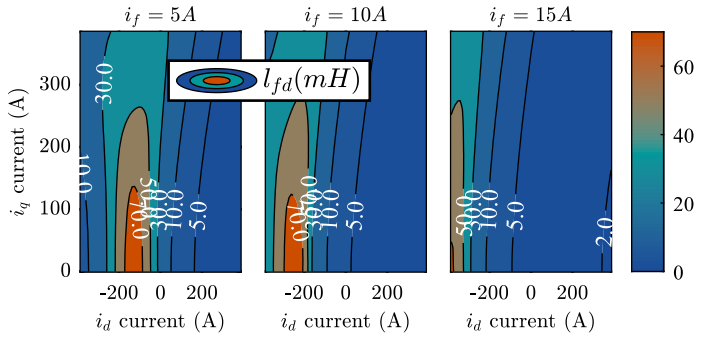
Fig. 23: Current-to-inductance l_{fd} map for the EESM under consideration.
