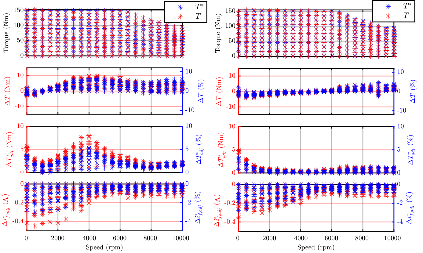
Fig. 30: Experimental results of steady-state torque accuracy using DB- dqs : (a) f_s = 3 kHz; (b) f_s = 10 kHz.
