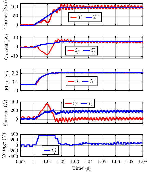
Fig. 24: Experimental results of torque transient response from 0 to 100 Nm, 5000 Nm/s, 4000 r/min using DB- dqs : view of the stator dq currents and the reference rotor voltage v_f^* .
