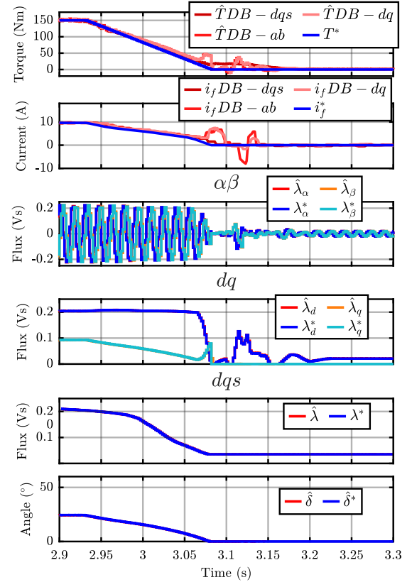
Fig. 28: Experimental results of torque transient from 150 to 0 Nm, 1000 Nm/s, 4000 r/min, f_s = 10 kHz (a downsampling of 1/20 is applied).
