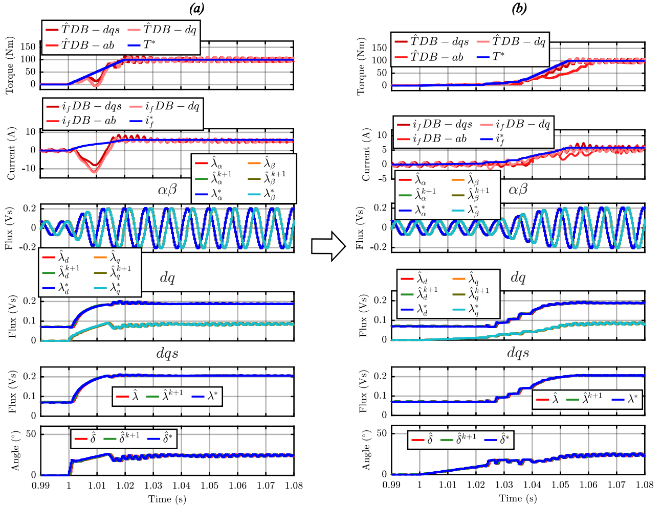
Fig. 21: Experimental results of torque transient response from 0 to 100 Nm, 5000 Nm/s, 4000 r/min: (a) without slew rate limitation for i_f < 1 A; (b) with slew rate limitation at 150 Nm/s for i_f < 1 A.
