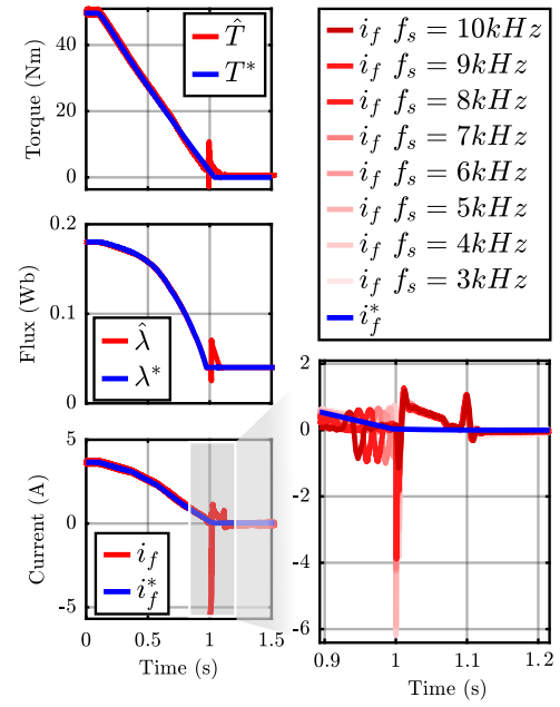
Fig. 27: Experimental results of torque transient from 50 to 0 Nm using DB-dqs, 50 Nm/s, 4000 r/min: effect of the sampling frequency.
