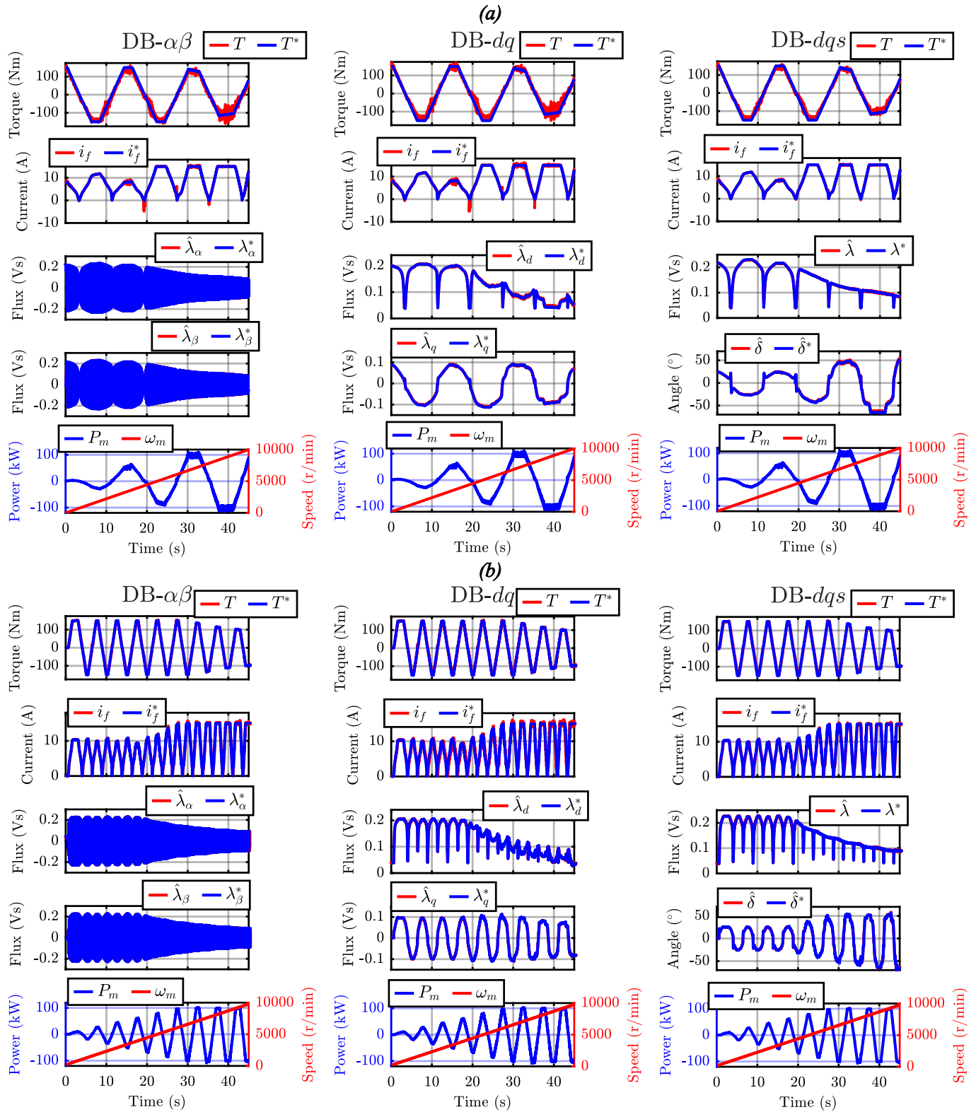
Fig. 29: Experimental results of fast torque reversals along the MTPS profile: (a) f_s = 3 kHz; (b) f_s = 10 kHz.
