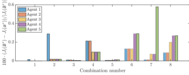
Fig. 4. Average cost variation at equilibrium, for each agent, w.r.t. the “nominal” one, i.e., \bar{x}^* , obtained by setting the matrix function A(\cdot) = I .
