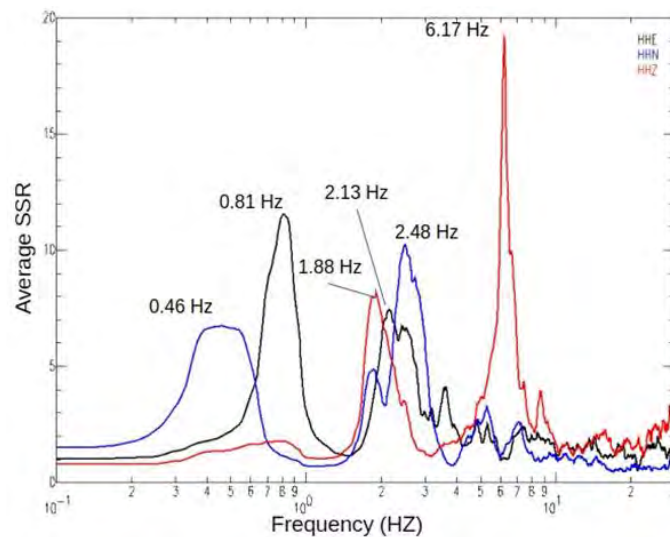
Figure 6. Frequencies of the main peaks on each component, averaged to obtain mean spectral ratios over all motion components, obtained from the SSR spectra of events with magnitude M \geq 4.0 .
