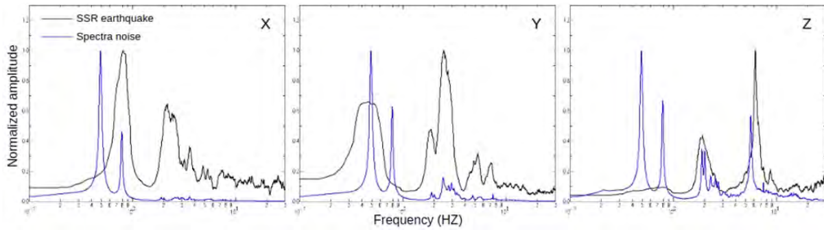
Figure 7. Comparison of mean SSR ratios on larger magnitude earthquakes and mean spectra calculated on free vibrations of the structure, calculated over approximately 50 consecutive days of recording.
