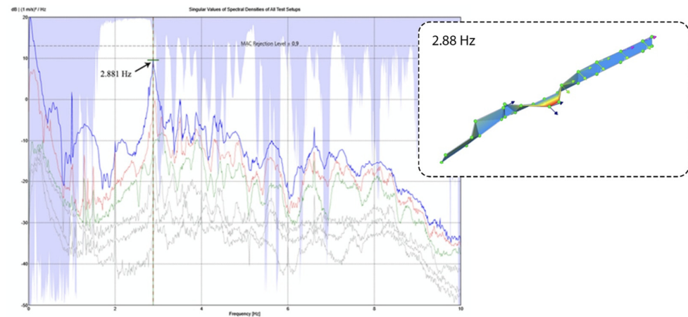
Figure 12. Average spectrum (FDD, in blue). The green dotted vertical line identifies the peak corresponding to the fundamental frequency, estimated at 2.88 Hz. The modal shape corresponding to the 2.88 Hz, the first modal frequency, is shown in the insert.
