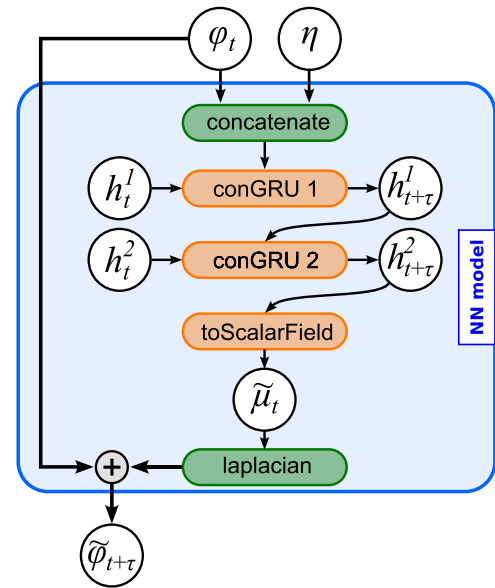
FIGURE 2 | Schematic representation of the Convolutional Recurrent NN model for evolution prediction. At each time step, the model predicts the time-evolved state \tilde{\varphi}_{t+\tau} from the previous state \varphi_t , the hidden states h_t^i and ( i enumerating the convolutional GRU submodule), and the parameter \eta provided as a constant field. Rather than predicting \tilde{\varphi}_{t+\tau} directly, the network outputs an auxiliary scalar field \tilde{\mu}_t , from which the updated state is computed. Green boxes represent fixed operations, while orange ones are learnable transformations.
