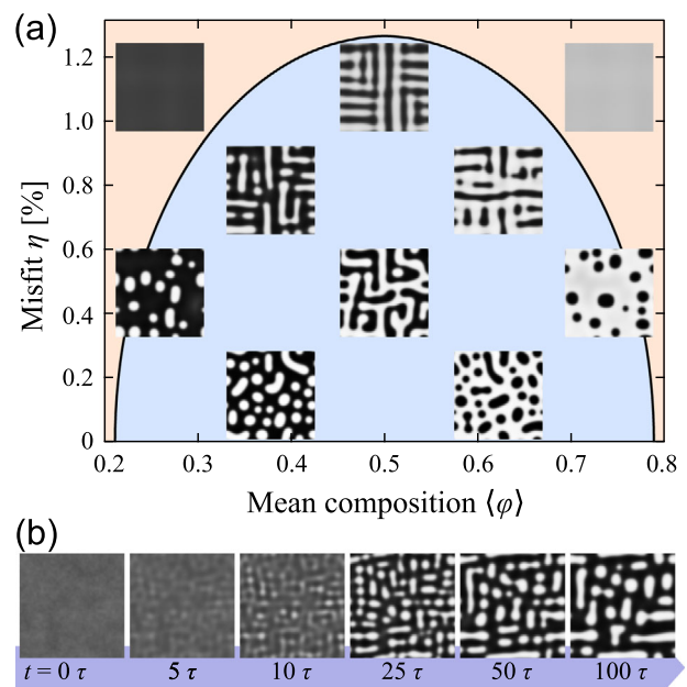
FIGURE 1 | (a) Phase diagram and examples of the different morphologies of the spinodal decomposition of a binary alloy with cubic elastic anisotropy, as a function of mean composition \langle\phi\rangle and misfit strain \eta . The reported images correspond to representative evolution stages obtained by the numerical integration of the Cahn–Hilliard Equation (8) starting from the homogeneous phase slightly perturbed by Perlin noise around the average composition \langle\phi\rangle . (b) Example of a phase-field evolution from the dataset, starting from a Perlin noise initial condition and corresponding to a misfit strain of \eta \approx 0.48\% .
