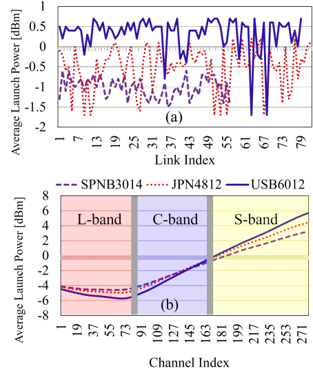
Fig. 11. The average launch power (a) per link is optimized with flat launch power (FLP), and (b) per links and channels is optimized with flat received power (FRP) in SPNB3014, JPNB4812, and USB6012.
