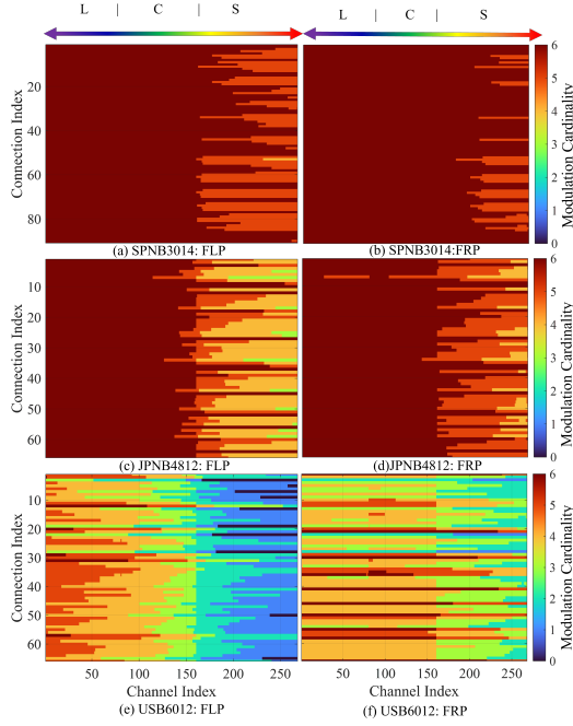
Fig. 10. Channel-connection capacity profile for the first candidate path in (a) SPNB3014-FLP, (b) SPNB3014-FRP, (c) JPNB4812-FLP, (d) JPNB4812-FRP, (e) USB6012-FLP, (f) USB6012-FRP. * to save space, we skip to show the channel-connection capacity profiles of the second and third shortest paths.
