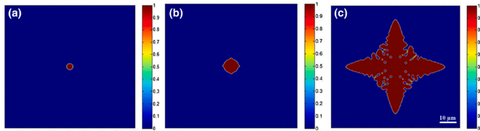
Fig. 7. Simulated dendrite structure growth at different times: (a) 0.01 ms, (b) 0.2 ms, and (c) 1.6 ms [161].
