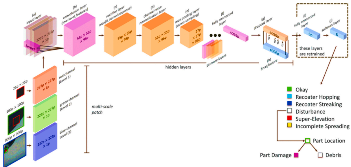
Fig. 9. Flowchart of implementing the MsCNN ML technique [234].
