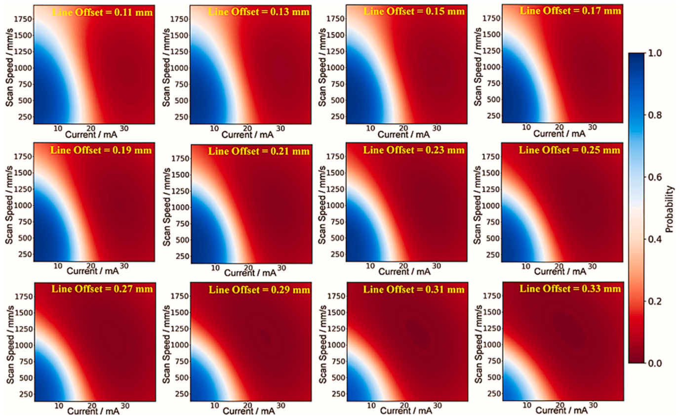
Fig. 15. Cross-sections of multidimensional process maps constructed using SVM as scan speed, current, and line offset functions. Dark blue (probability: 1.0) indicates that the surface morphology of the part printed by the processing parameters is predicted to be a good (even) surface without internal defects, and dark red (probability: 0.0) indicates a bad (uneven or porous) surface with internal defects [283]. (For interpretation of the references to color in this figure legend, the reader is referred to the web version of this article.)
