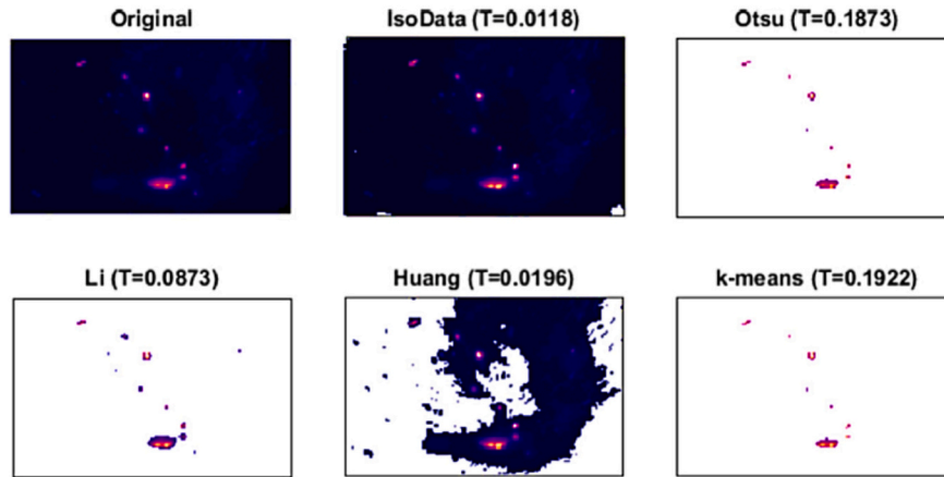
Fig. 12. Example of an IR image where only the LHZ and the spatters are evident, and Segmentation results based on IsoData, Otsu's, Li's, Huang's, and k-means methods [264].
