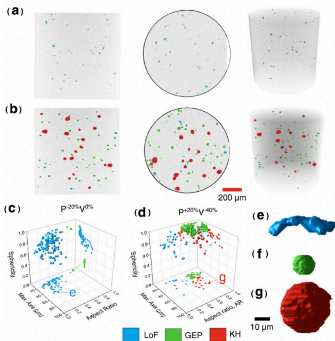
Fig. 11. Visualization of volumetric defects in L-PBF coupons. Front, top, and isometric views of the XCT scan region of coupons fabricated using (a) P - 20% V0% and (b) P + 20%V - 40% parameters. Scatterplots in the 3D space of size, aspect ratio, and sphericity show the volumetric defects observed in (c) P - 20%V and (d) P + 20%V - 40% coupons. Appearances of selected defects, (e) a LoF, (f) a GEP, and (g) a KH-Induced porosities, are also shown [48].
