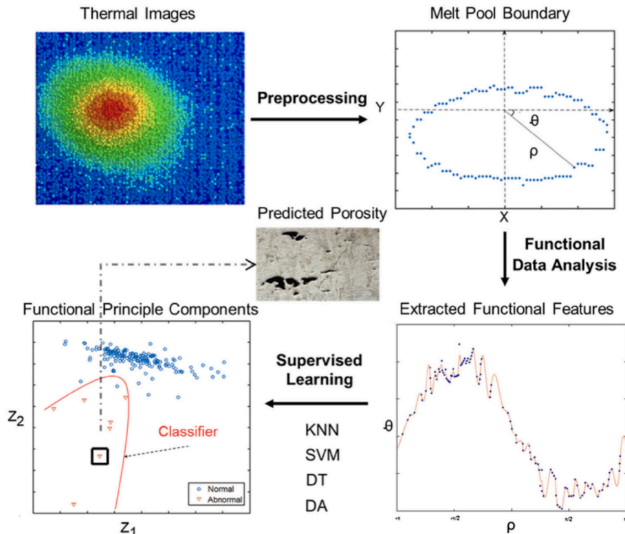
Fig. 10. Demonstration of porosity prediction using supervised machine learning [250].
