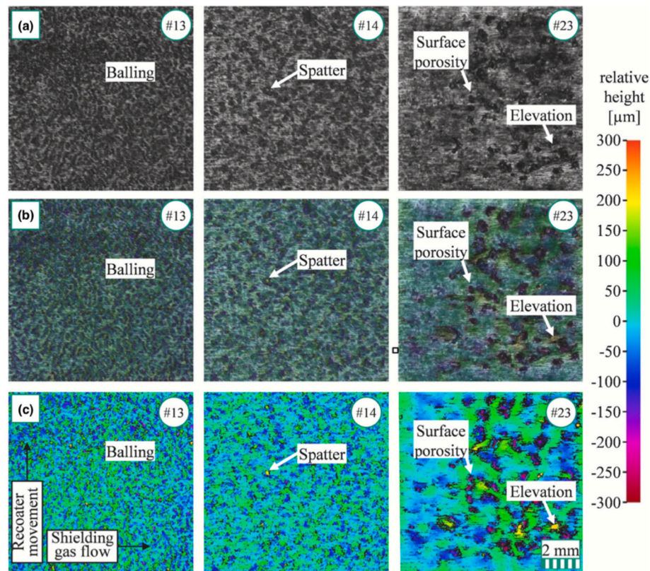
Fig. 2. Surface images of samples produced in the experiment: (a) captured in-situ using the camera system, (b) both superimposed images, and (c) a topographical image acquired ex-situ using an Alicona Infinite Focus, where “0” indicates the mean plane [56].
