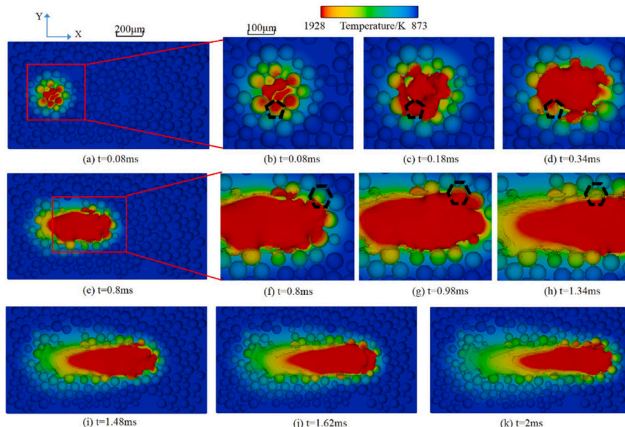
Fig. 8. Simulation results of the formation process of a nonuniform single track [201].
