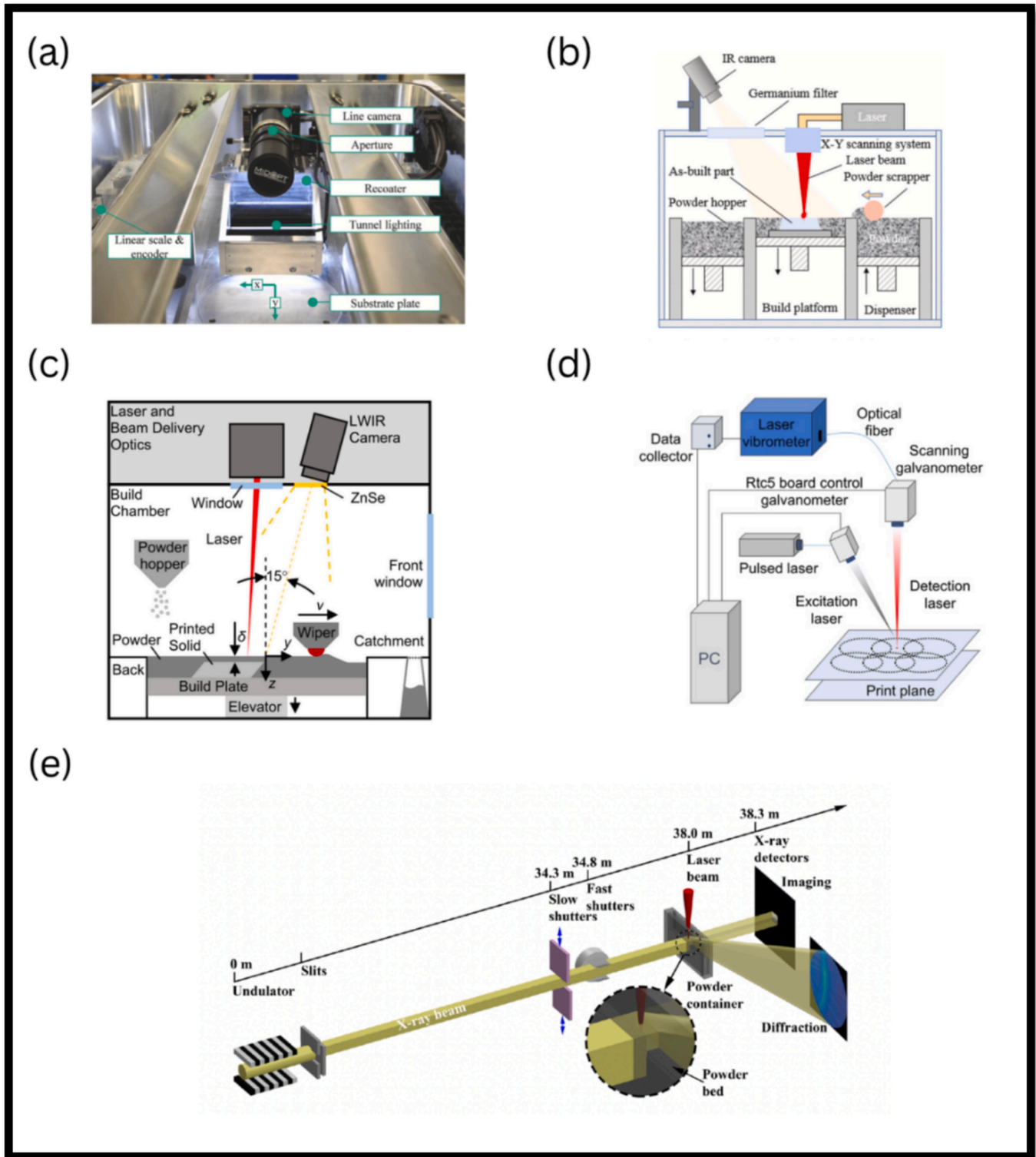
Fig. 4. (a) Optical monitoring system integrated into an L-PBF machine [56]. (b) Schematic diagram of the IR monitoring system integrated into the L-PBF experimental setup [64]. (c) Illustration of the L-PBF experimental setup, including the LWIR camera [90]. (d) Multi-circle scanning using a laser ultrasonic system [77]. (e) Schematic of the high-speed X-ray imaging and diffraction setup for L-PBF at the Advanced Photon Source [91].
