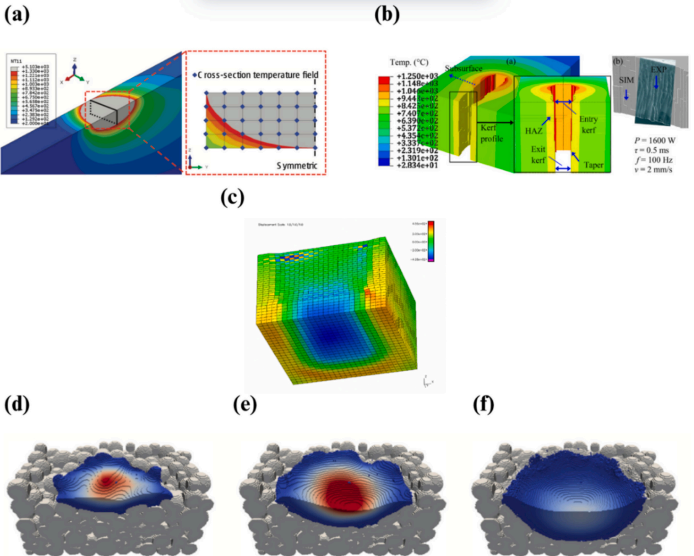
Fig. 5. (a) Temperature field in the cross-section of laser scanning track [106], (b) Representative prediction of laser cut kerf and comparison between predicted and measured striated surfaces [105], (c) Cube example after 12 layers deposited, Tzz stress [MPa] [107], (d) Snapshots of spot melting in a powder bed at different time steps; the beam pulse duration in 2500-time steps, (e) 5000-time steps (f) 10,000-time steps [108].
