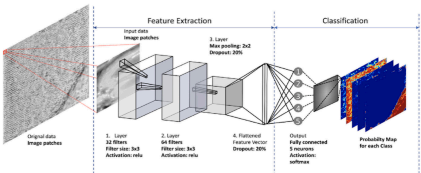
Fig. 14. The architecture of the proposed CNN model is used to predict surface roughness and defective areas [277].
