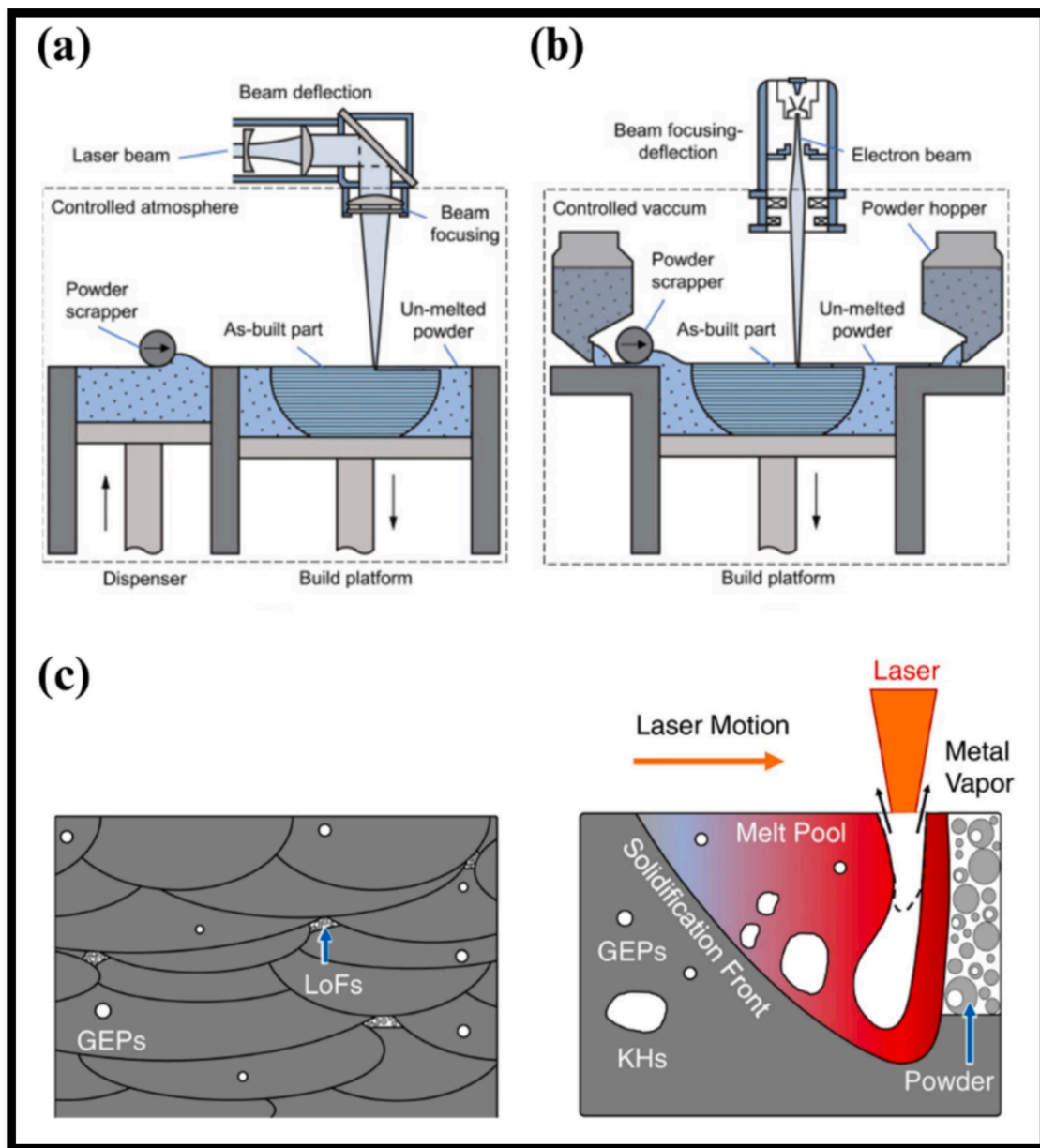
Fig. 1. The schematic illustration of two PBF machines: (a) L-PBF and (b) EB-PBF [47]. (c) Explanation of the formation of various defects in L-PBF [48].
