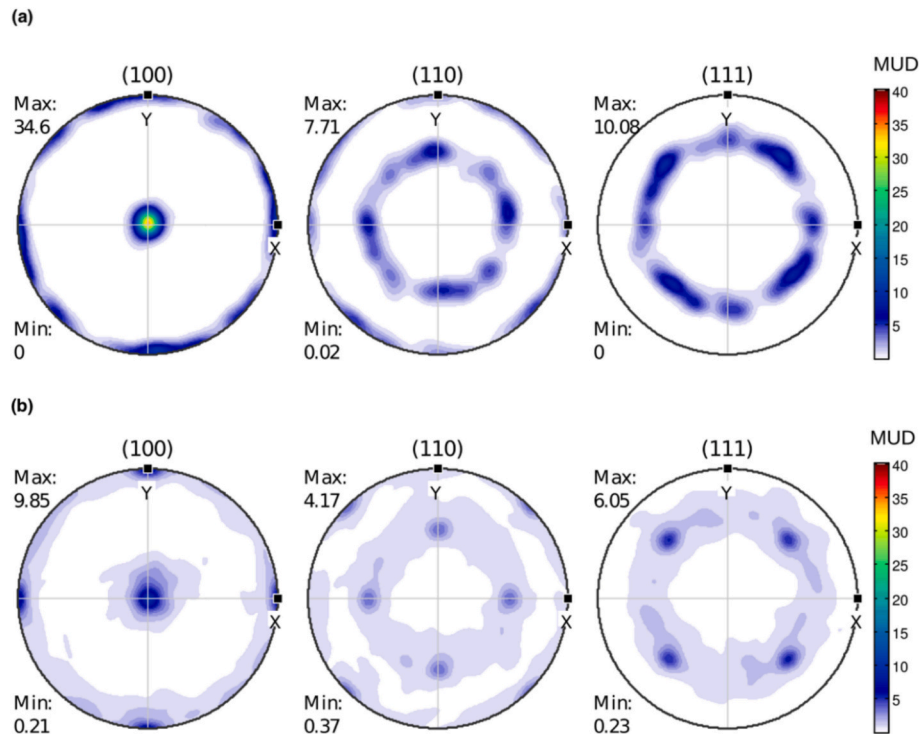
Fig. 6. Representative pole figures in the XY-plane: (a) Columnar grains. Parameters: EA = 1.8 \text{ J mm}^{-2} , v = 2.2 \text{ ms}^{-1} , L_{off} = 150 \text{ } \mu\text{m} , (b) Equiaxed grains. Parameters: EA = 1.9 \text{ J mm}^{-2} , v = 8.8 \text{ ms}^{-1} , L_{off} = 1/437.5 \text{ mm} [126].
