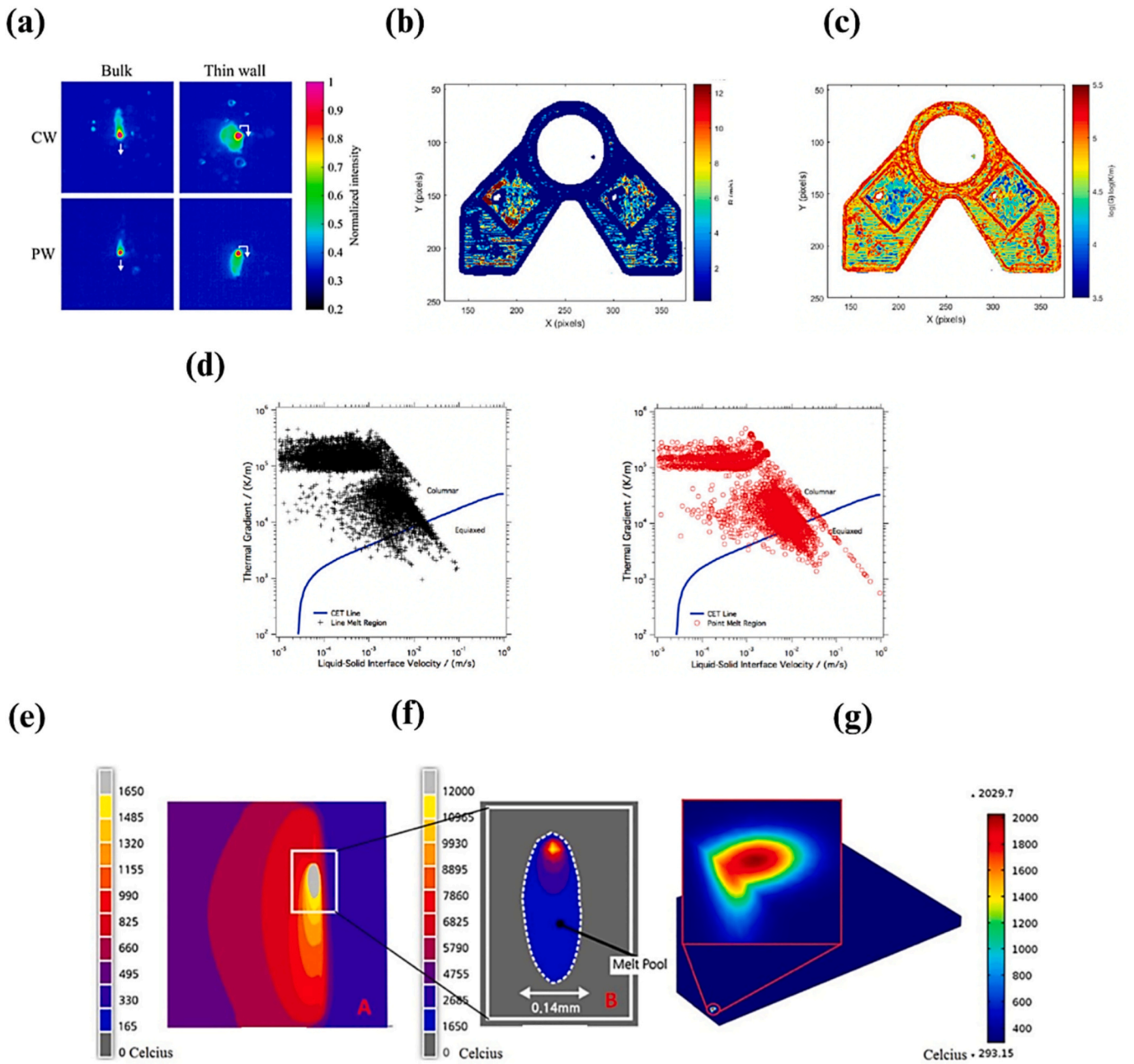
Fig. 3. (a) NIR images captured for both bulk and thin wall geometries under various emission modes. White arrows highlight the beam trajectory [70]. The layer Thermal Gradients (b), Interface Velocity (c), and CET curve (d) [71]. Performing precision process of thermal measurement (e, f); Zoomed-in melt pool geometry and temperature distribution (g) [69].
