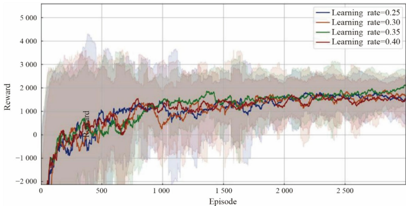
Fig. 9 Effects of the learning rate on the accumulated final reward for a target melt pool depth of 0.3 mm
