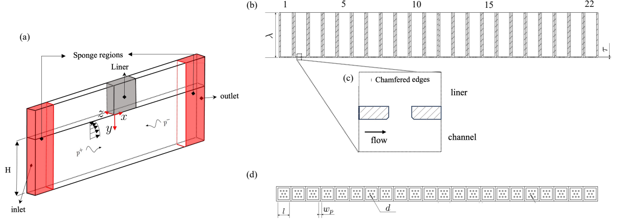
Fig. 1 Sketch of the numerical setup (a) 3D geometry, (b) 2D cross-plane of the acoustic liner, (c) sketch of the orifice shape, (d) facesheet detail of the liners.
