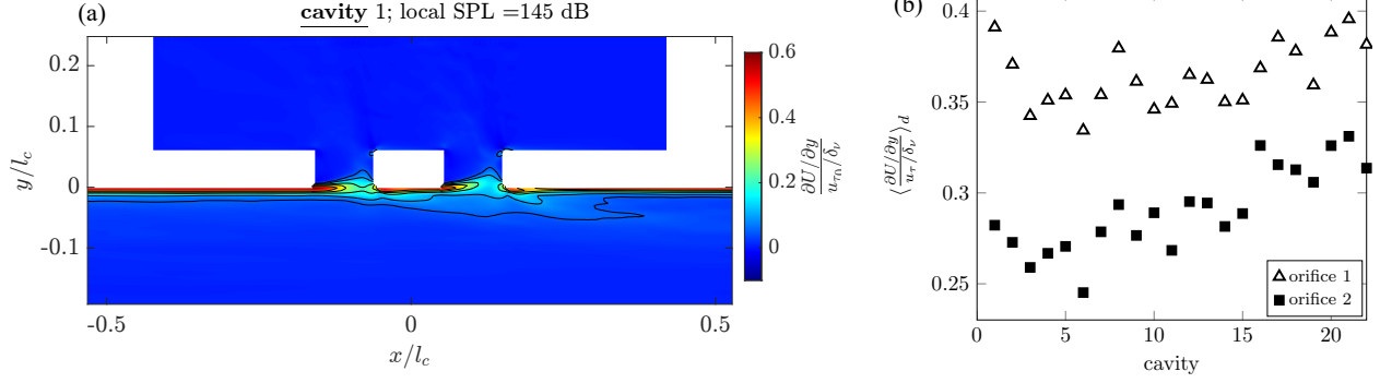
Fig. 5 Normalized shear layer over the cavity, (a) contour on the first cavity, (b) averaged normalized shear over the diameter for the first and second orifice as function of the cavity number.
