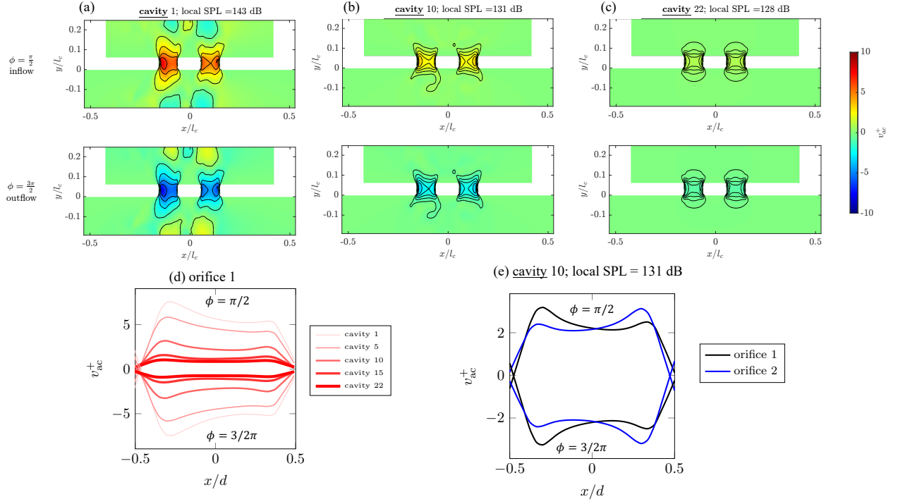
Fig. 3 Contour of the wall-normal acoustic induced velocity v_{ac}^+ in inflow and outflow phases at M = 0 , forcing frequency equal to 1400 Hz, incident SPL = 145 dB \phi , (a) cavity 1, (b) cavity 10, (c) cavity 22; v_{ac}^+ profiles at various phases taken at the centreline of the orifice (d) first orifice, effect of changing the cavity (e) cavity 10, comparison between orifice 1 and 2.
