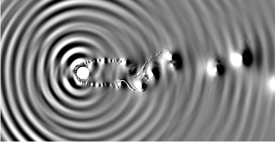
Fig. 6 Instantaneous snapshot of the dilation field \partial p / \partial t induced by a cylinder covered with an SPC.
