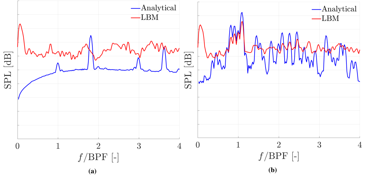
Fig. 14 Pressure fluctuations in dB at r_1/D = 2.15 and \varphi = 0 at max efficiency. (a): EB/EV. (b): UB/UV.
