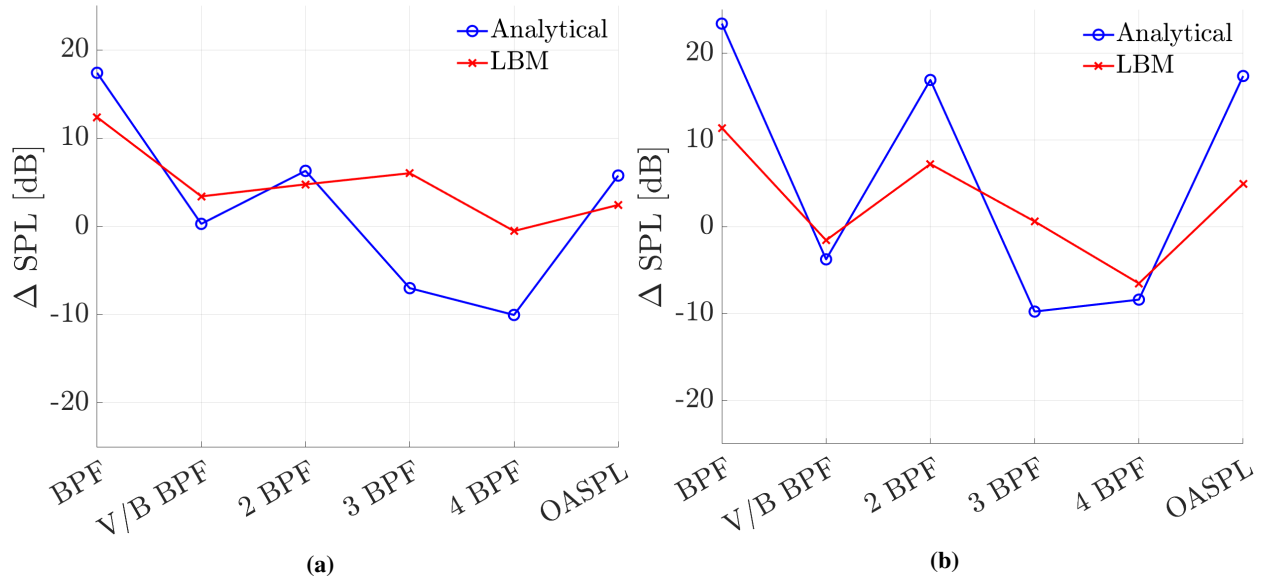
Fig. 15 Narrowband SPL difference between the UB/UV and EB/EV configurations for a far-field probe located at r_1/D = 2.15 and \varphi = 0 . (a): Free blowing. (b): Max efficiency.
