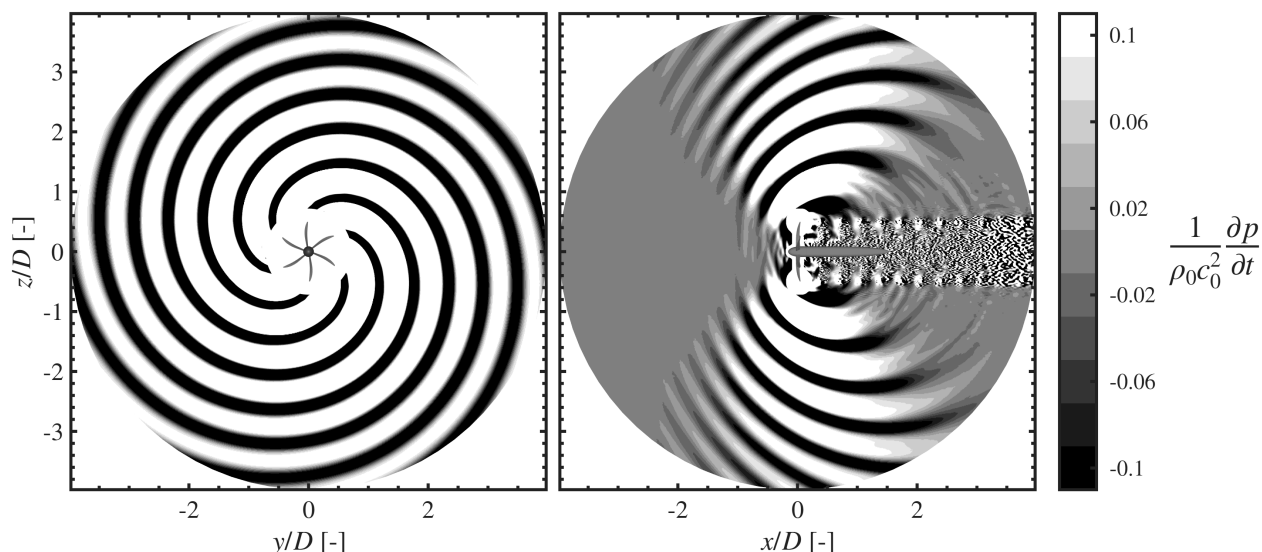
Figure 5: Dilatation field around the propeller obtained from direct CFD data.
