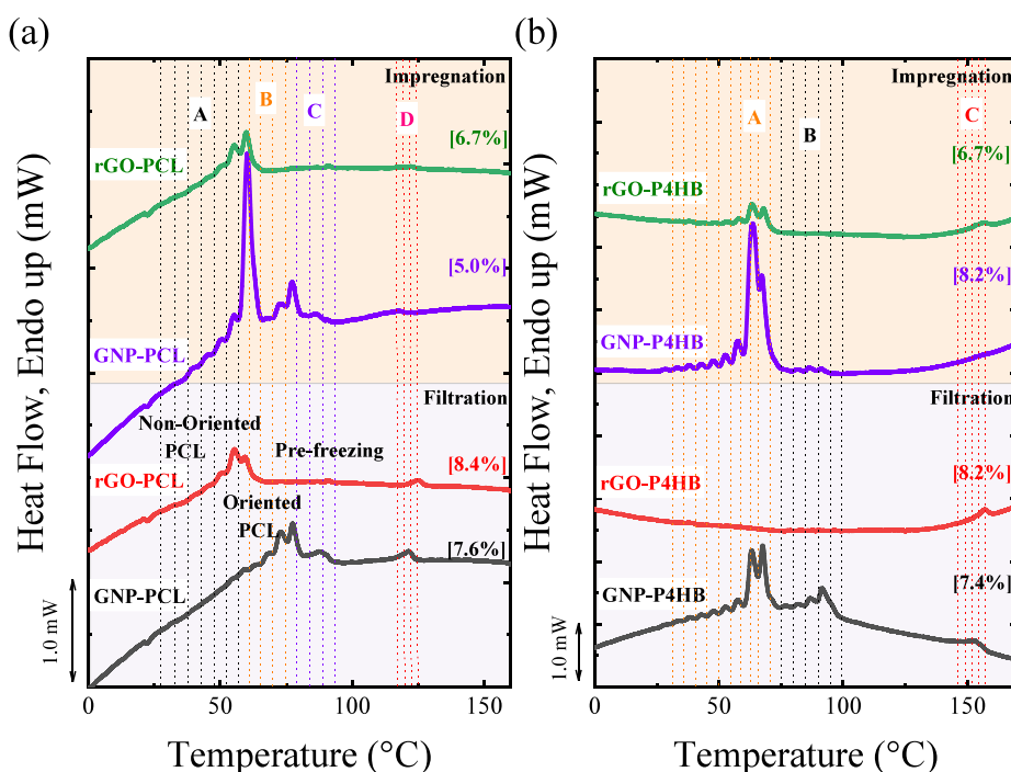
Figure 5. Final DSC heating curves after SSA of PCL and P4HB nanopapers prepared by different methods and different GRMs: (a) PCL, (b) P4HB. In brackets are the polymer contents from TGA (Figure S2).
