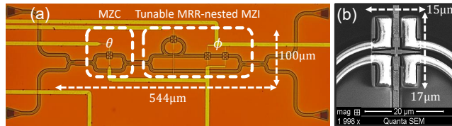
Figure 1: (a) Micrograph of the NLA device. The tunable MZC is followed by a MRR nested on a MZI; (b) Detailed SEM magnification of the ultra-compact PS available on the IMOS platform.
