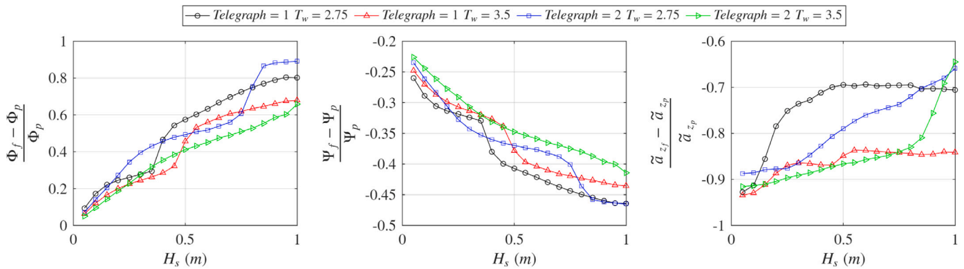
Fig. 16. Relative variance of speed-keeping, specific fuel consumption, and vertical acceleration performance of the hydrofoil configuration compared to the planing baseline. The comparative metrics are plotted against significant wave height for selected telegraph and wave period combinations.
