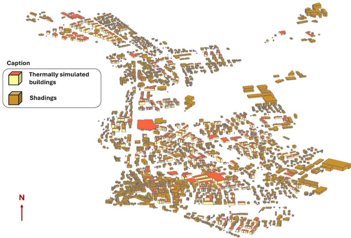
Fig. 3. Whole URBEM for the city of Monthey.
