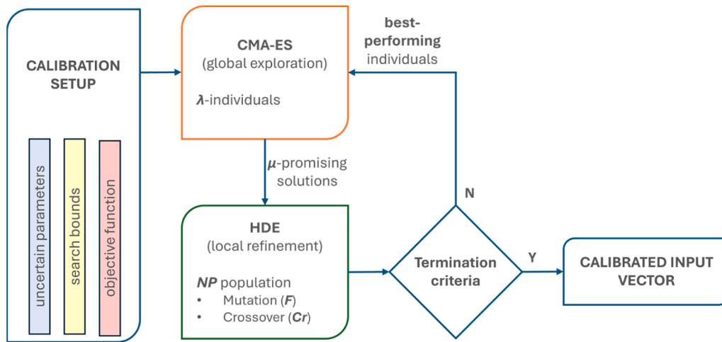
Fig. 2. Conceptual workflow of the hybrid CMA-ES/HDE calibration framework used for UBEH parameter optimisation.
