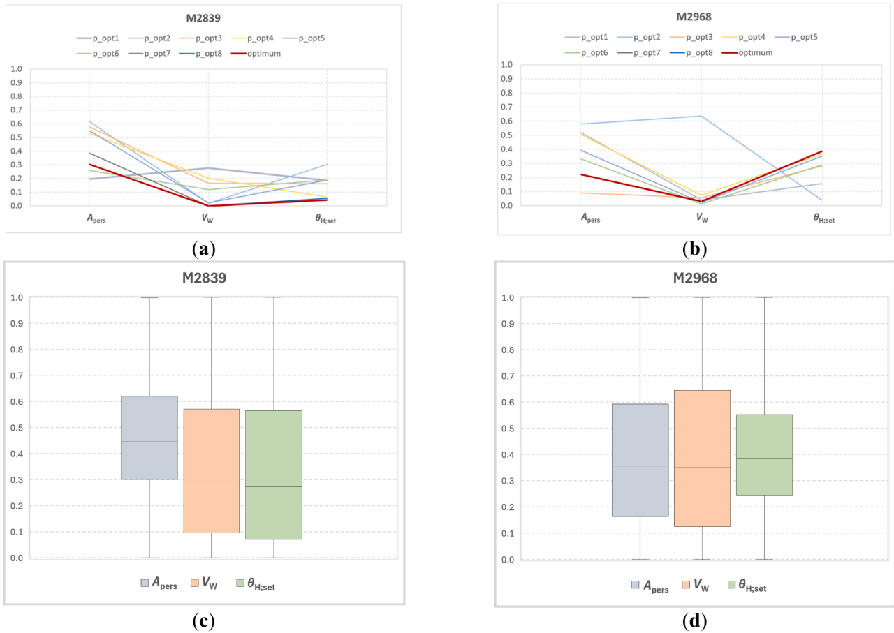
Fig. 13. Urban block M2839: partial and global optima and full distribution of simulated inputs, for M2839 (a-c) and M2968 (b-d) multi-family houses, respectively.
