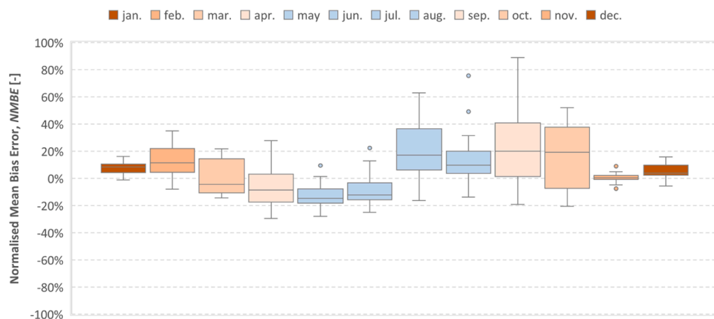
Fig. 11. Temporal distribution of monthly NMBE for calibrated residential buildings built in 1961–70.
