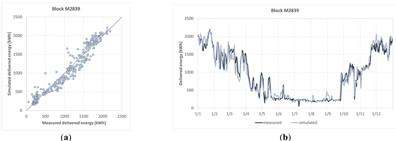
Fig. 14. Daily measured vs simulated delivered energy for urban block M2839: measured-simulated (a) and time-series comparison (b).
