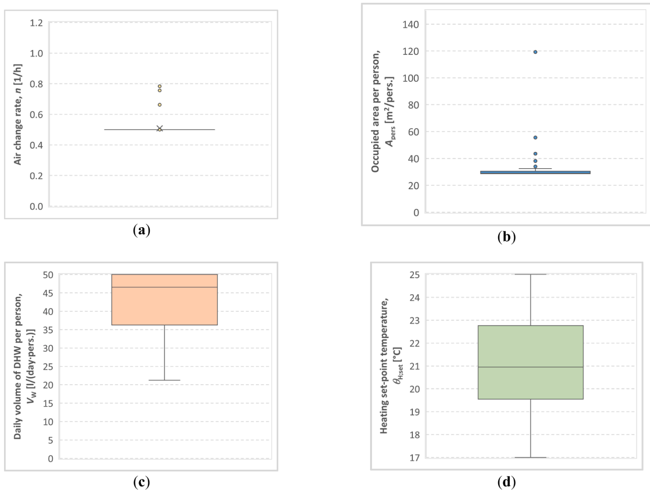
Fig. 10. Boxplots of input variables after calibration process for multi-family houses: air change rate (a), occupied area per person (b), daily volume of DHW per person (c), and heating set-point temperature (d).
