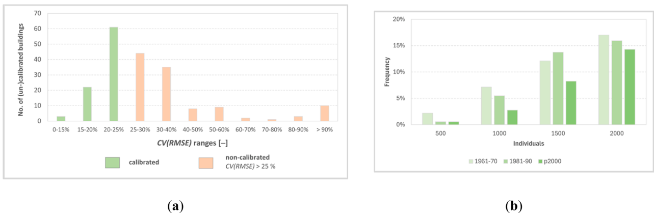
Fig. 9. Distribution of CV(RMSE) ranges across the (un-)calibrated buildings (a); frequency of case studies with CV(RMSE) \leq 25\% across individual classes, by construction period (b).
