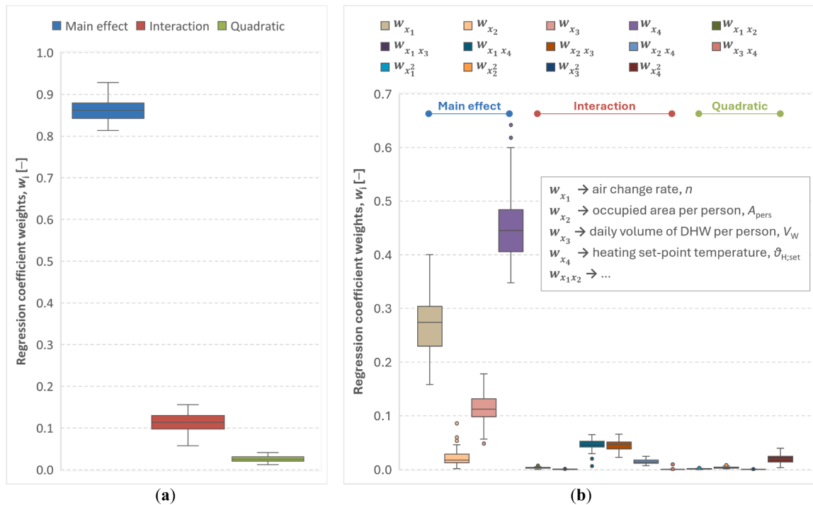
Fig. 12. Weights of regression coefficients for residential buildings constructed in 1961–70: aggregated by main, interaction, and quadratic effects (a), and disaggregated by independent variables (b).
