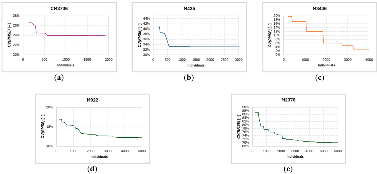
Fig. 8. Evolution of CV(RMSE) values during the calibration process for various case studies: at the building-scale (a), and at the block-scale with 2 buildings (b), 3 buildings (c), 4 buildings (d), and 5 buildings (e).
