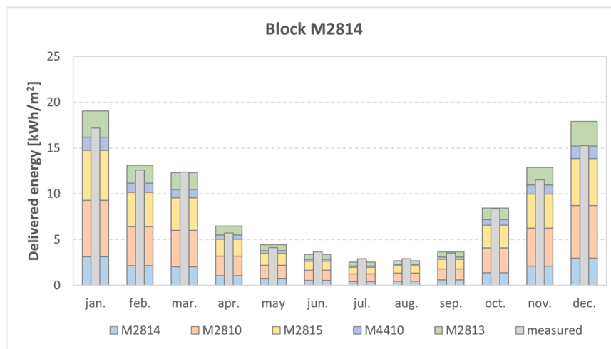
Fig. 15. Monthly delivered energy intensity for the urban block M2814, expressed in kWh/m 2 . The stacked columns represent the simulated contributions of the individual buildings (M2814, M2810, M2815, M4410, and M2813), while the adjacent grey column indicates the measured energy consumption for each month.
