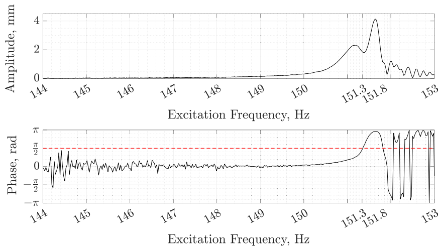
Fig. 12. ODS amplitude and phase evolution obtained from CHF method as functions of excitation frequency.
