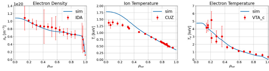
Fig. 5. Experimental (red) and simulated (blue) profiles for discharge #41279 (H-mode). Electron density and temperature profiles are compared to Thomson scattering signals. For the former the signal is fitted with the IDA algorithm [23], for the latter, signal directly from the diagnostic (VTA in AUG [24]) is used. Ion temperature is compared with the charge exchange recombination spectroscopy (CUZ in AUG).
