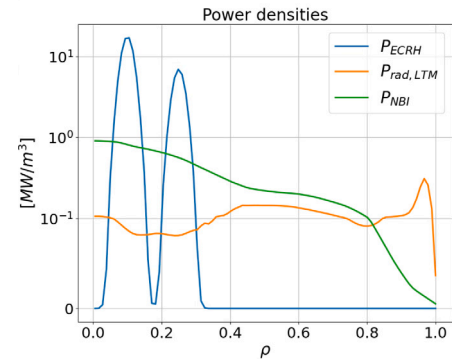
Fig. 9. Comparison of injected power from both NBI and ECRH system, and radiated power emitted from Sn by the LTM.
