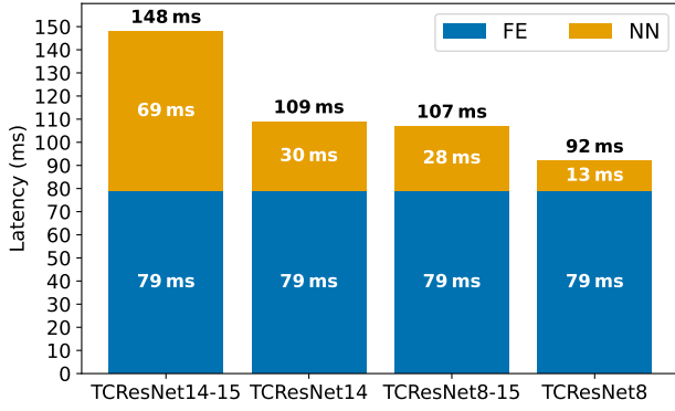
Fig. 1. Front-end (FE) and neural network (NN) latency breakdown in KWS pipelines built with the TC-ResNet model family on an STM32F767ZI MCU.
