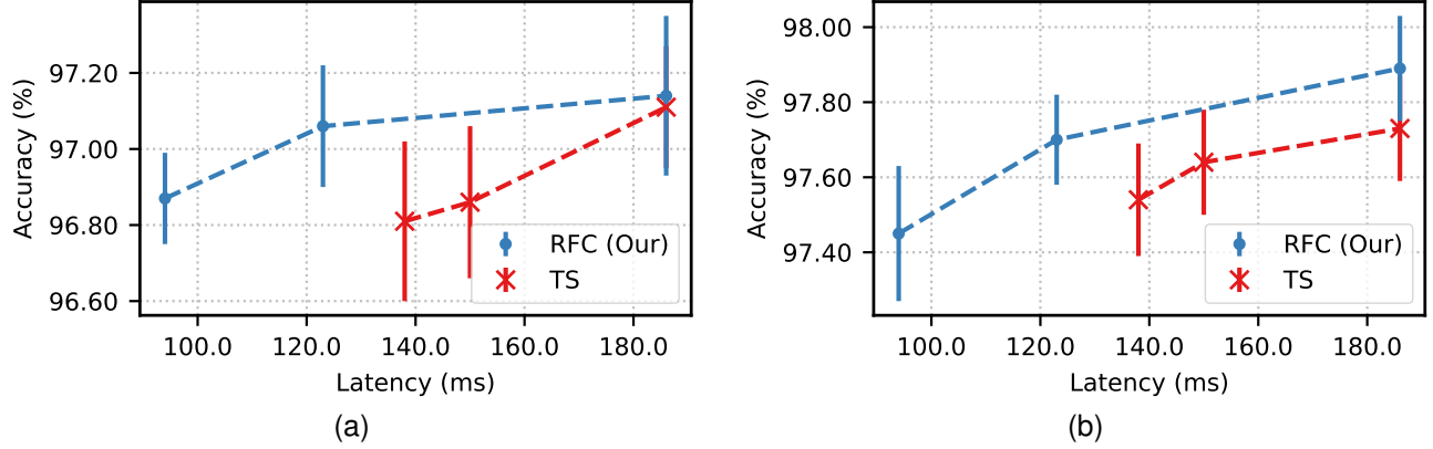
Fig. 7. Accuracy vs. Latency with Topology Scaling (TS) and RFC on an STM32F767ZI MCU. Results for MatchboxNet on (a) GSCv1 and (b) GSCv2.
