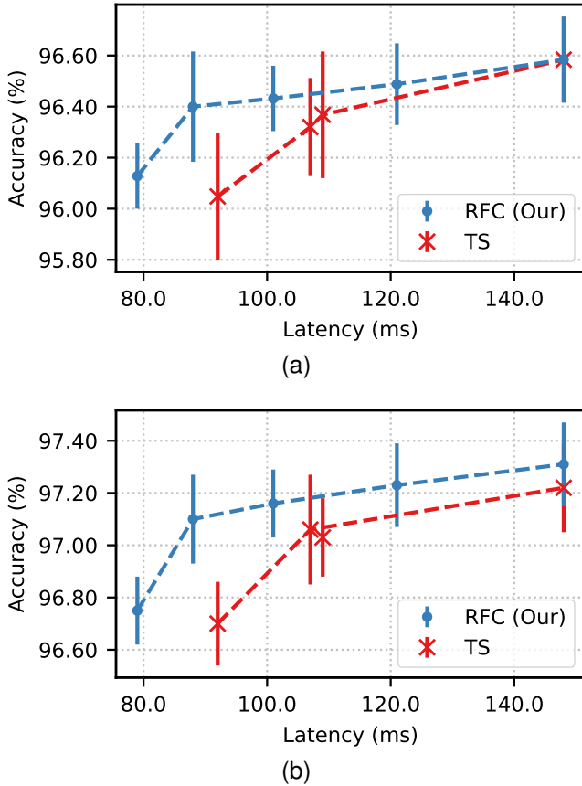
Fig. 6. Accuracy vs. Latency trade-offs obtained with Topology Scaling (TS) and RFC with five operating modes on an STM32F767ZI MCU. Results on (a) GSCv1 and (b) GSCv2.
