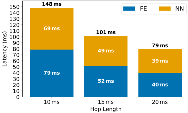
Fig. 4. KWS Latency using TC-ResNet-14-15 with different hop lengths on an STM32F767ZI MCU.
