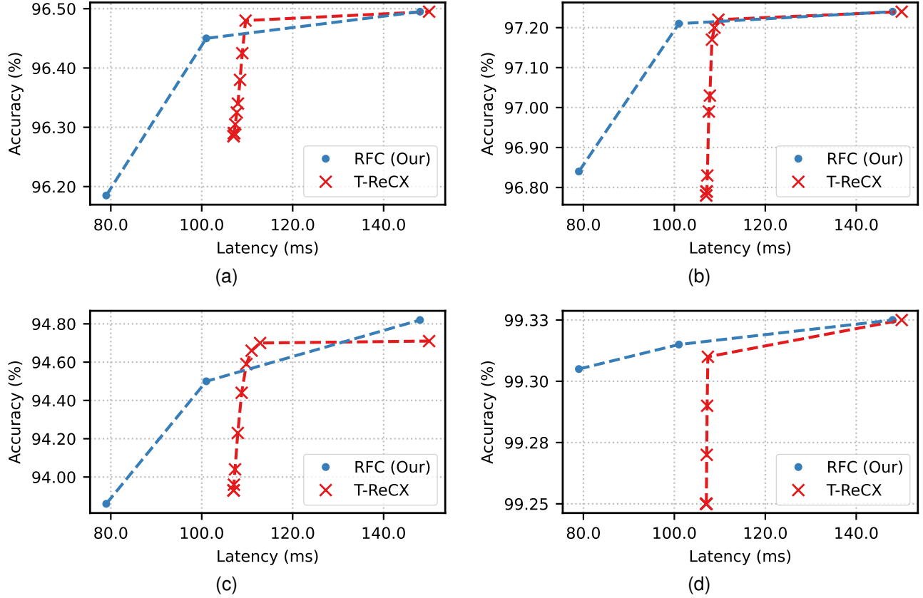
Fig. 5. Accuracy vs. Latency trade-offs obtained with early-exit (T-ReCX [28]) and the proposed Runtime Feature Compression (RFC) on an STM32F767ZI MCU. Results on (a) GSCv1, (b) GSCv2, (c) MSWC, (d) Hey Snips.
