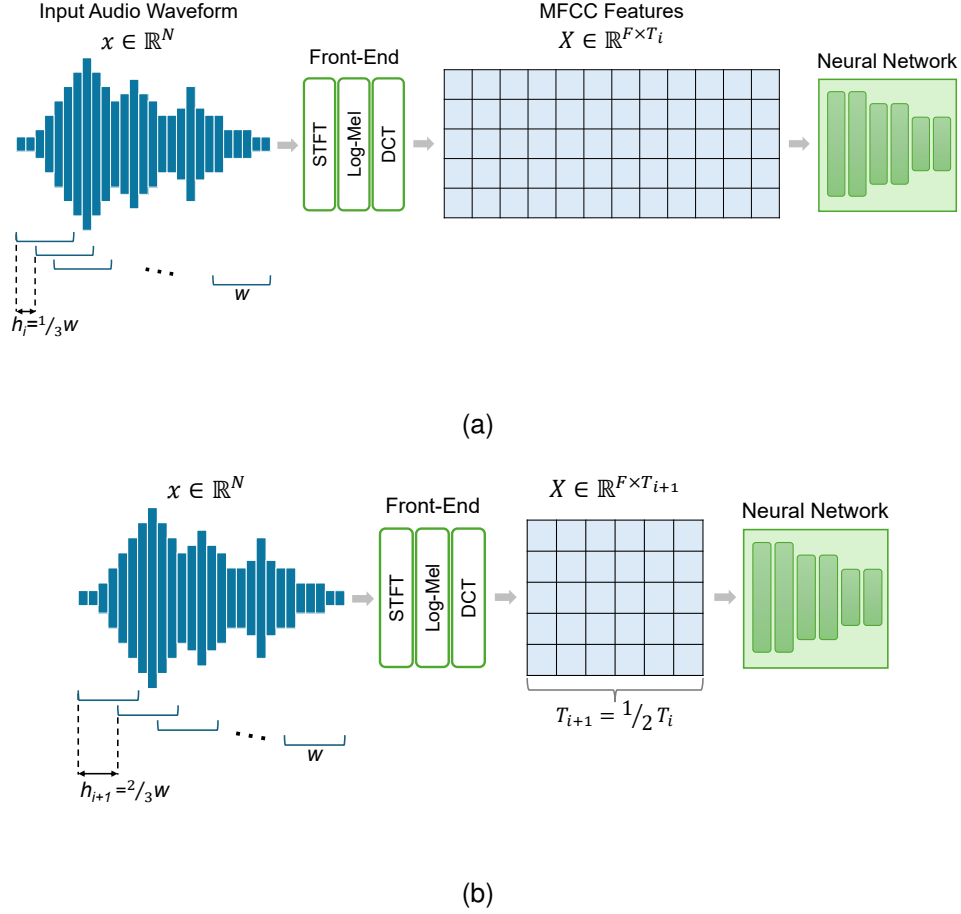
Fig. 2. Schematic overview of the proposed Runtime Feature Compression (RFC) mechanism. RFC introduces the STFT hop length h as a runtime control knob to modulate the temporal dimension of audio features, and hence the computational complexity of both the front-end and the classification stages.
