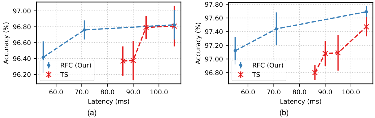
Fig. 8. Accuracy vs. Latency with Topology Scaling (TS) and RFC on an STM32F767ZI MCU. Results for TENet on (a) GSCv1 and (b) GSCv2.
