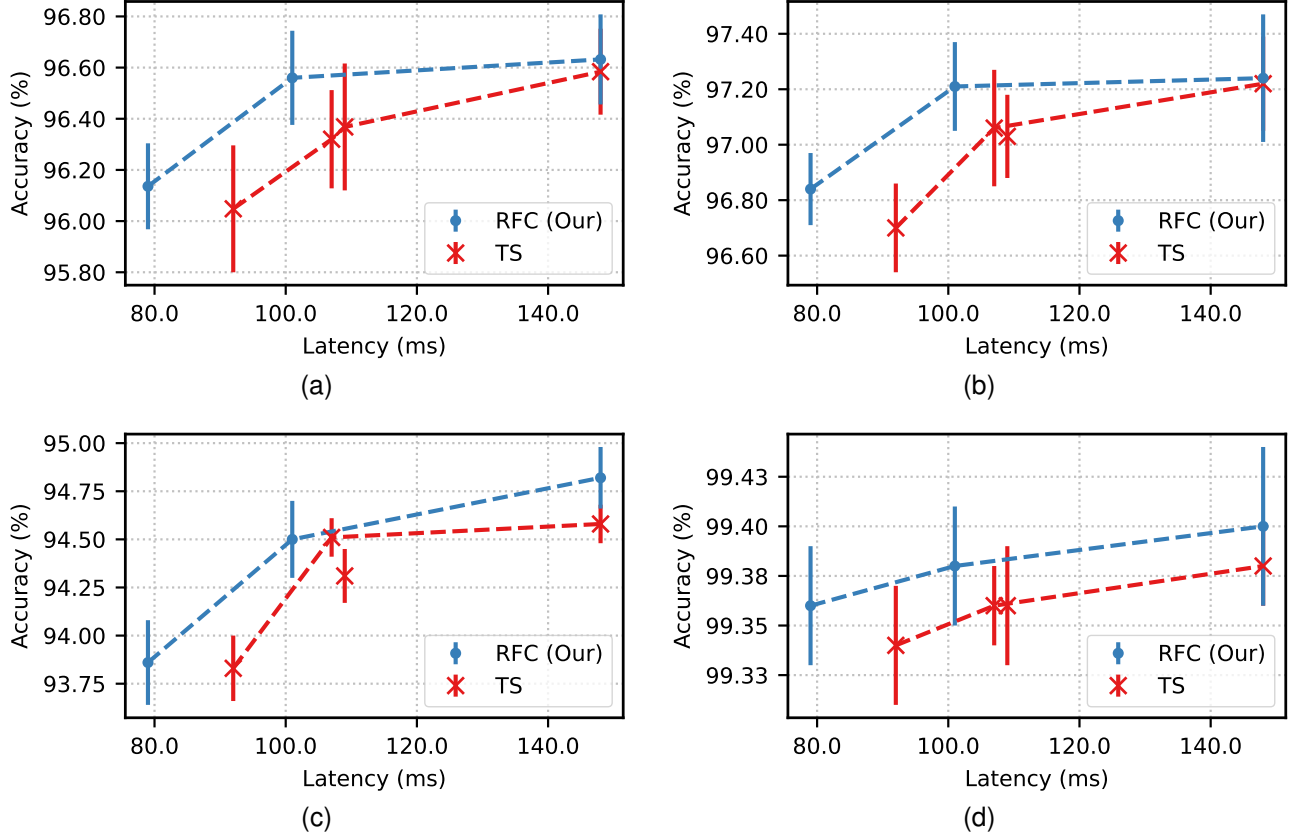
Fig. 3. Accuracy vs. Latency trade-offs obtained with Topology Scaling (TS) and the proposed Runtime Feature Compression (RFC) on an STM32F767ZI MCU. Results on (a) GSCv1, (b) GSCv2, (c) MSWC, (d) Hey Snips.
