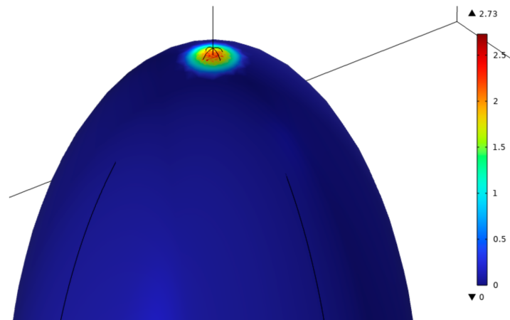
Figure 16. Case study 2: map of \epsilon_{ep} at void tip for E_{\text{appl}} = 203 kV/m.
