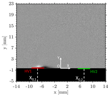
Fig. 4. Schlieren image after the background subtraction; in white, the reference system adopted. The high-voltage electrodes HV 1 and HV 2 have been marked with red and green lines, respectively. X_{0,1} and X_{0,2} represent the centers of HV 1 and HV 2 respectively. Images have been cropped to focus on the region of interest (For interpretation of the references to colour in this figure legend, the reader is referred to the web version of this article.).
