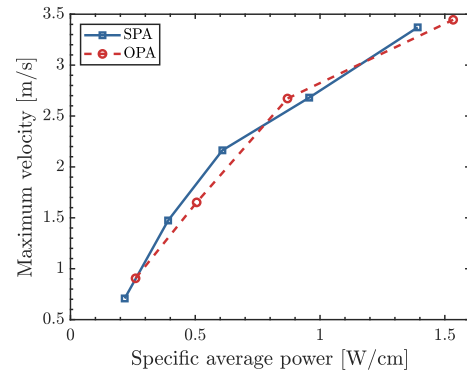
Fig. 16. Maximum induced velocity as a function of the specific average power for the large-scale and lab-scale SPAs.
