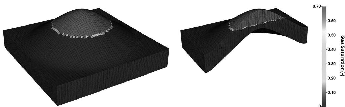
Fig. 1 – View of the 3D model with the adopted gridding and the distribution of the initial gas saturation for the reservoir base case (model A).
