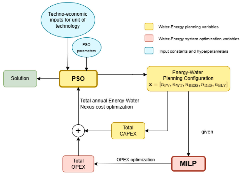
Fig. 1. Optimization flow for energy–water planning using PSO-MILP framework.
