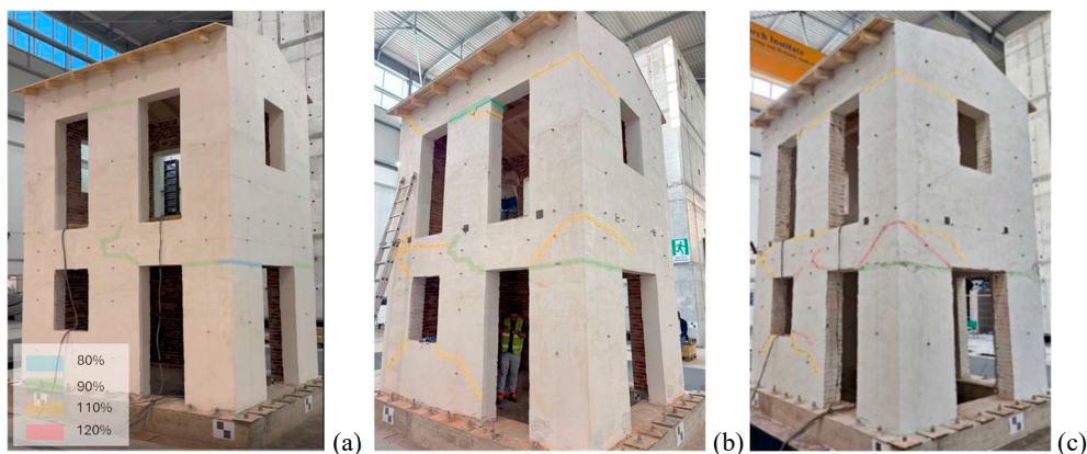
Fig. 6. Crack patterns at the end of the sequential shakings: (a) AB; (b) EFS; (c) EFS+RW
