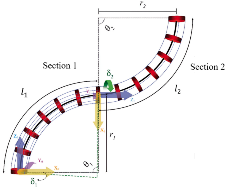
Fig. 1. Schematic of the two-segment continuum robot (Jabari et al., 2025).
