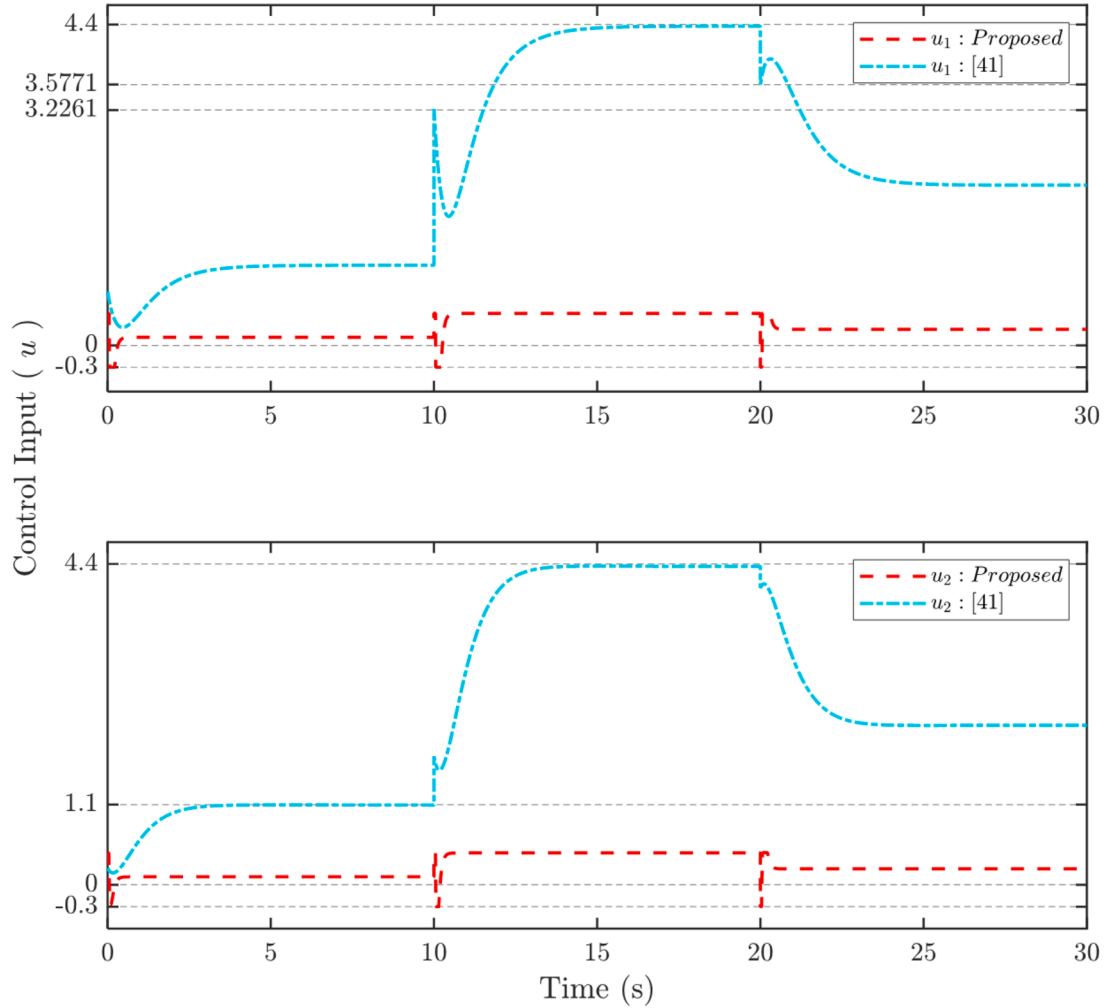
Fig. 5. Comparison of control inputs under step signal.
