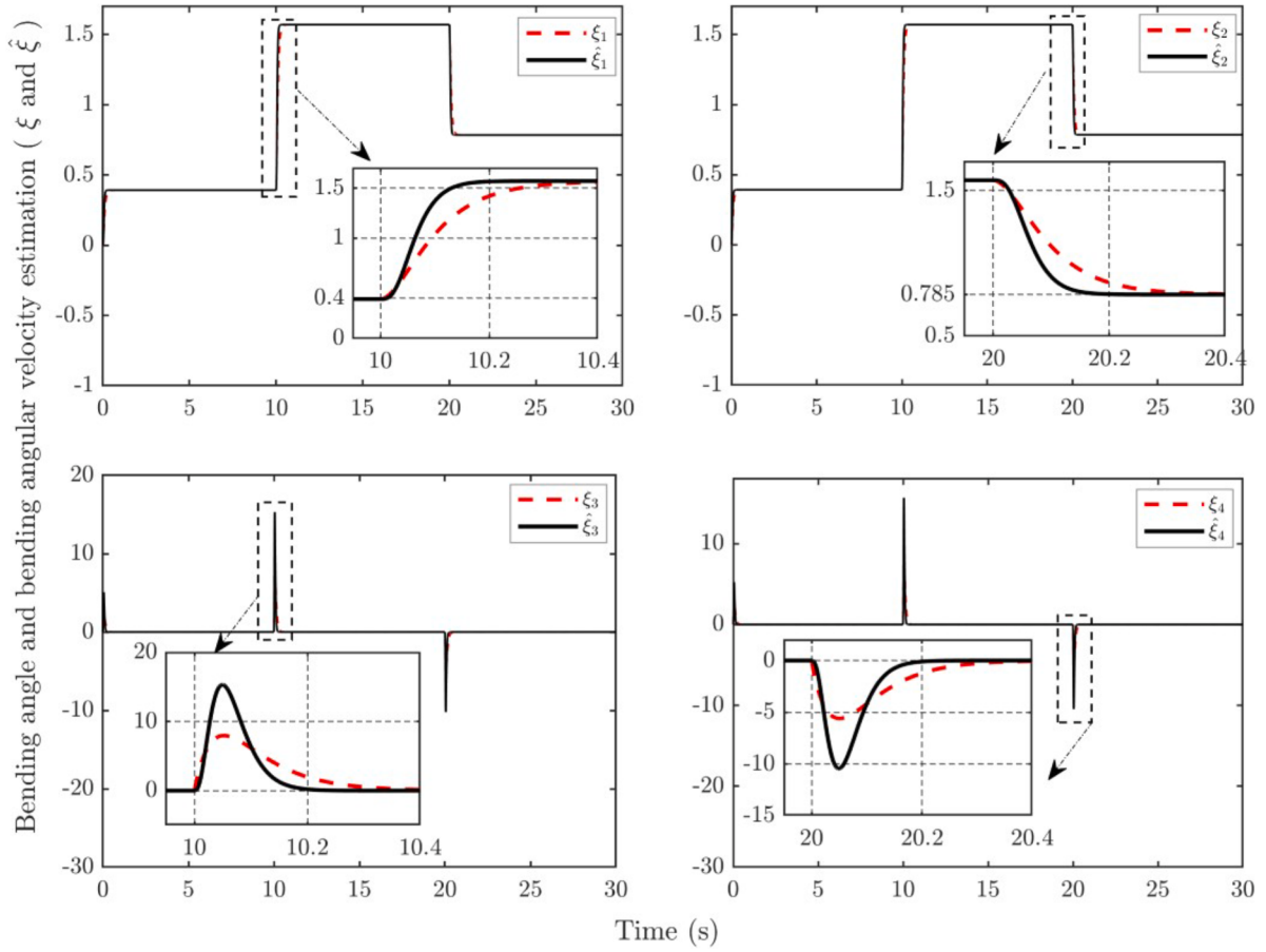
Fig. 6. Dynamic variables of the continuum robot system and their estimated values under step signal.
