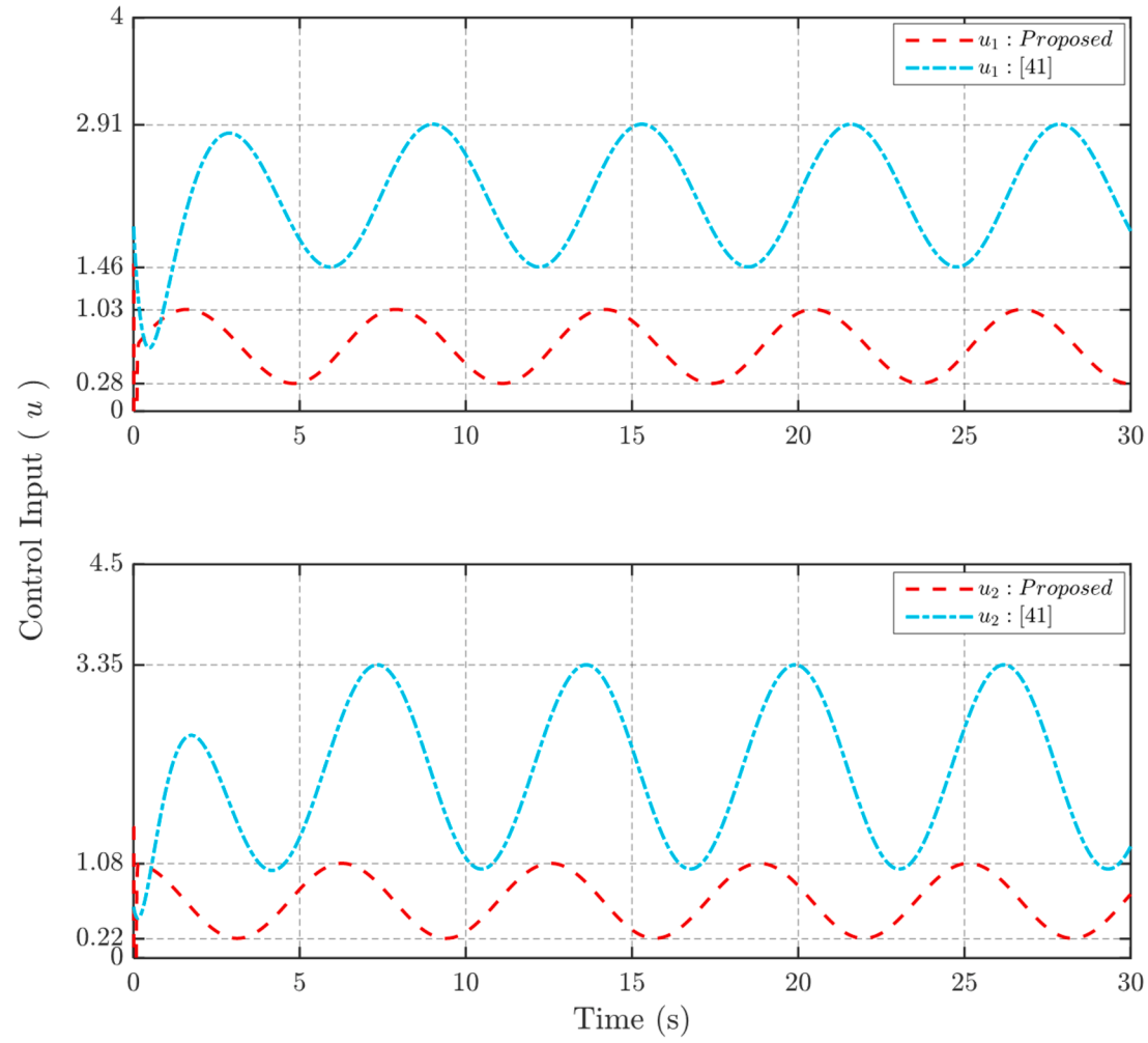
Fig. 9. Comparison of control inputs under Sinusoidal signal.
