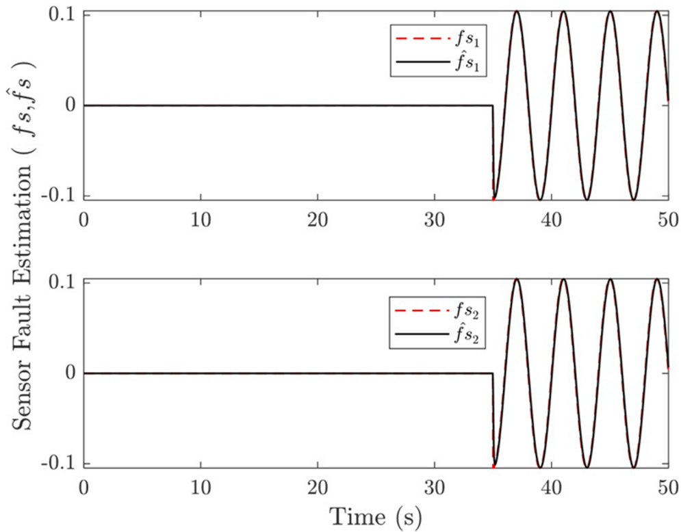
Fig. 13. Sensor faults estimation.
