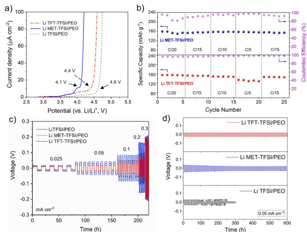
Fig. 2 Electrochemical behavior of Li TFT-TFSI/PEO (red), Li MET-TFT/PEO (blue), and Li TFSI/PEO (black) at 70 °C: (a) linear sweeping voltammetry profiles measured in a \text{Li}^+|\text{Li}_x/\text{PEO}||\text{Al} carbon-coated configuration at a scan rate of 0.1 \text{ mV s}^{-1} ; (b) specific capacity and coulombic efficiency as a function of cycle number for \text{Li}^+|\text{Li}_x/\text{PEO}||\text{LiFePO}_4 cells at variable C-rates; (c) galvanostatic cycling of \text{Li}^+|\text{Li}_x/\text{PEO}||\text{Li}^+ symmetric cells at different current densities (total plated/stripped capacity of 0.3 \text{ mAh cm}^{-2} per half cycle); (d) long-term cycling performances of Li symmetric cell at 0.050 \text{ mA cm}^{-2} .
