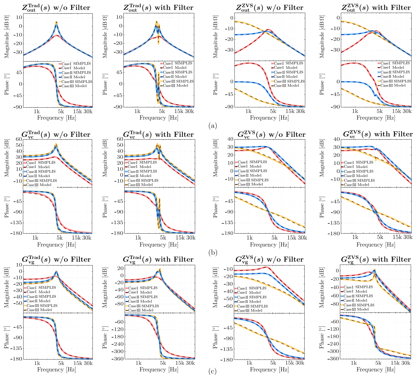
FIGURE 8 | TFs comparison without and with the EMI filter for both traditional and QSW-ZVS designs: (a) output impedance Z_{\text{out}}^v(s) , (b) control-to-output transfer function G_{vc}^v(s) , and (c) line-to-output transfer function G_{vg}^v(s) .
