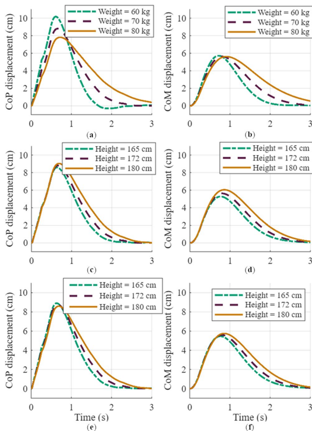
Fig. 9 CoP_m and CoM dependence from weight (a, b) and height (c–f) of the subject (body height set at 172 cm). In c and d the distance between the perturbation application point and the ankle joint was maintained proportional to the subject's height (body weight set at 70 kg); while in e and f the perturbation was always applied at a distance of 126 cm from the ankle (body weight set at 70 kg)
